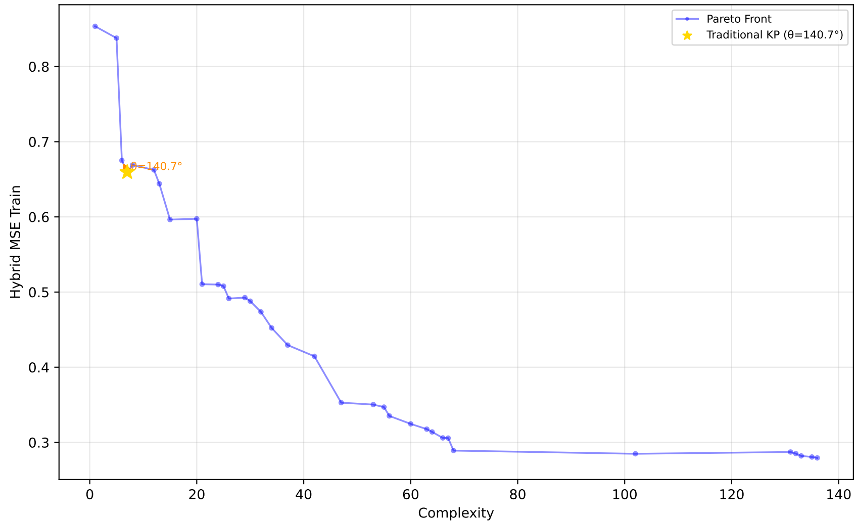
522_pm10 - Run 30 - SVP - Hybrid MSE Train \lambda_1=1.00, \lambda_2=0.00, \lambda_3=0.90 | Difficulty: 1.00 | Method: hmr
