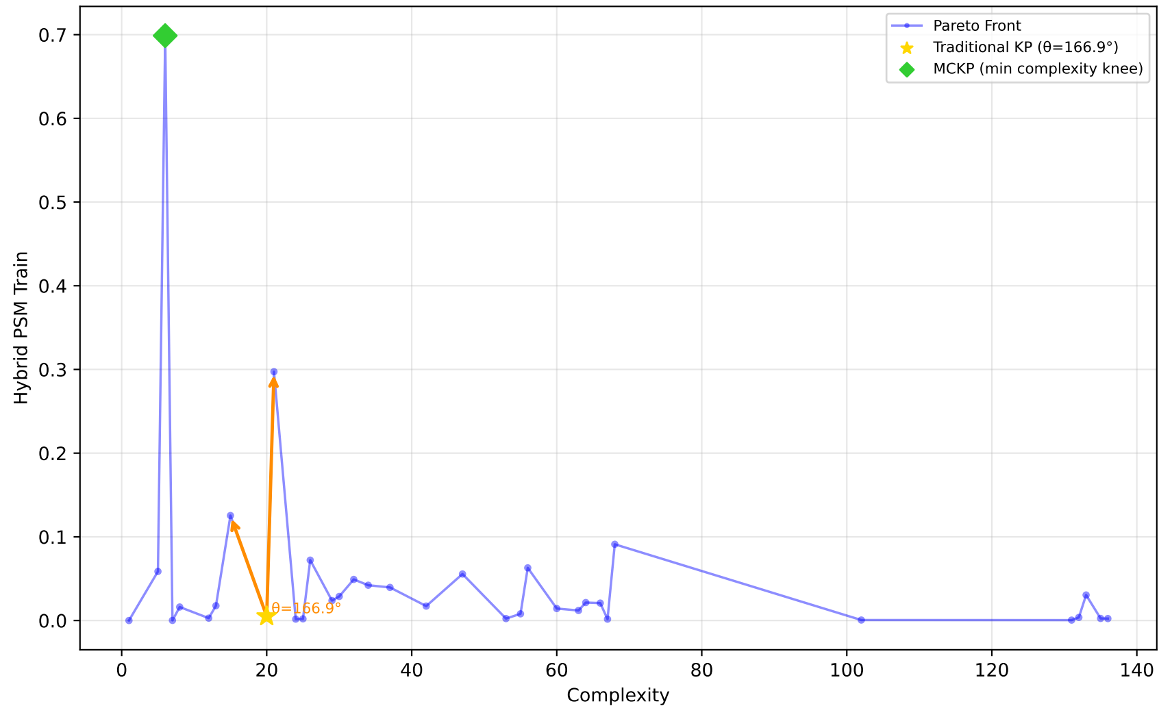
522_pm10 - Run 30 - SVP - Hybrid PSM Train \lambda_1=0.00, \lambda_2=0.10, \lambda_3=0.00 | Difficulty: 1.00 | Method: hmr
