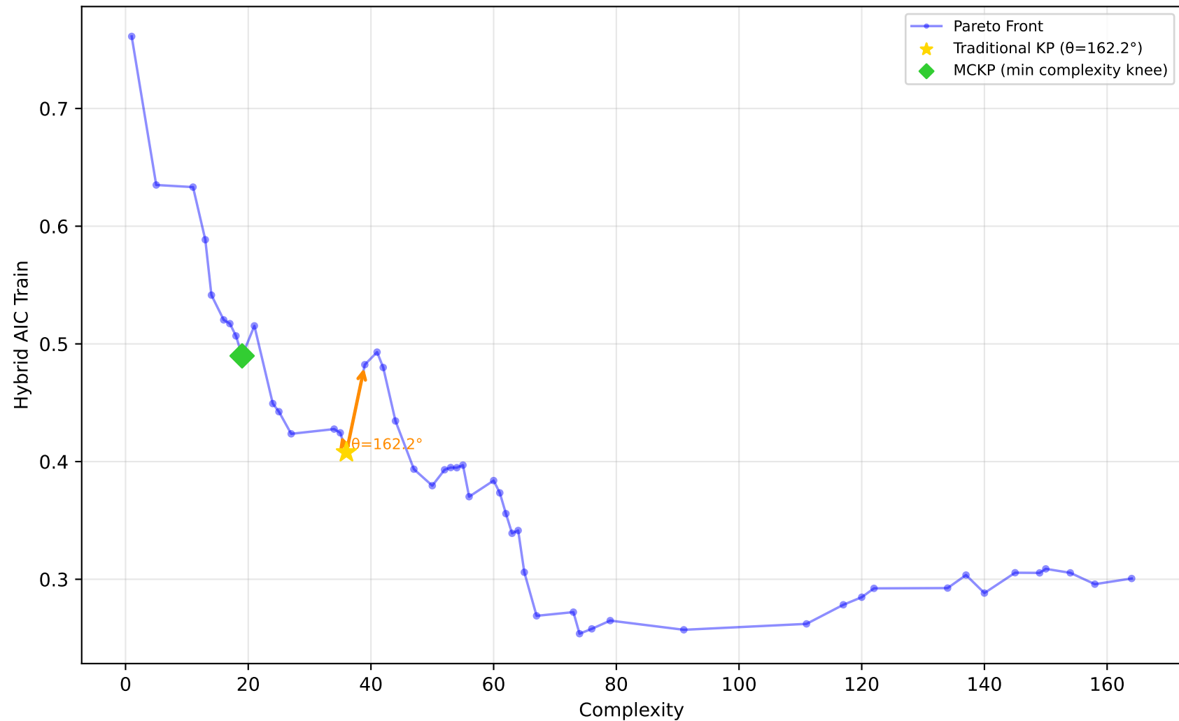
522_pm10 - Run 3 - MVP - Hybrid AIC Train \lambda_1=1.00, \lambda_2=0.00, \lambda_3=0.00 | Difficulty: 1.00 | Method: hmr
