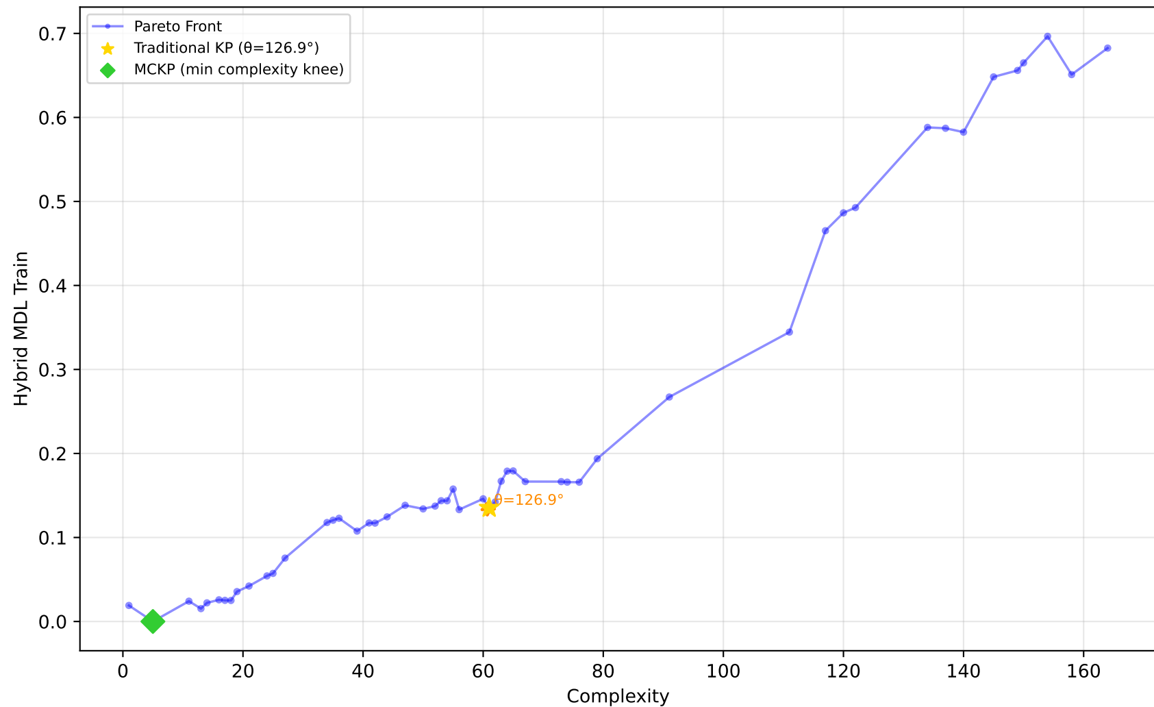
522_pm10 - Run 3 - MVP - Hybrid MDL Train \lambda_1=0.00, \lambda_2=0.90, \lambda_3=0.00 | Difficulty: 1.00 | Method: hmr
