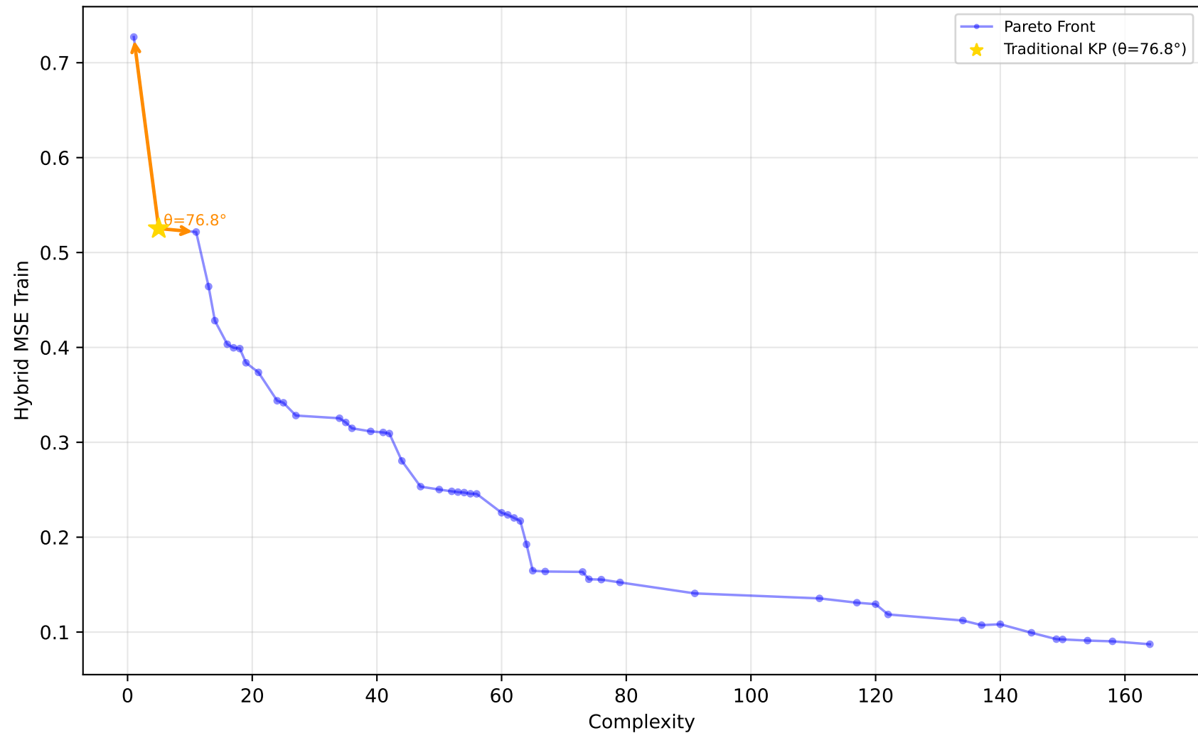
522_pm10 - Run 3 - MVP - Hybrid MSE Train \lambda_1=0.00, \lambda_2=0.90, \lambda_3=0.00 | Difficulty: 1.00 | Method: hmr
