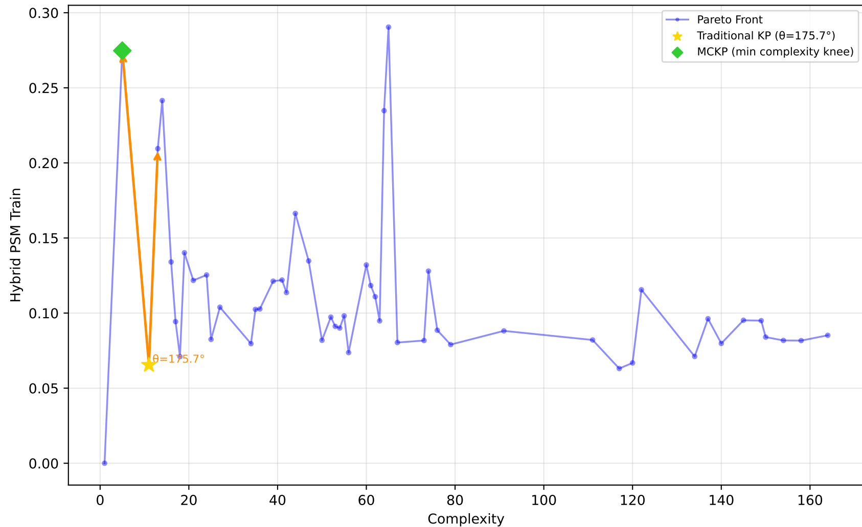
522_pm10 - Run 3 - MVP - Hybrid PSM Train \lambda_1=1.00, \lambda_2=0.00, \lambda_3=0.00 | Difficulty: 1.00 | Method: hmr
