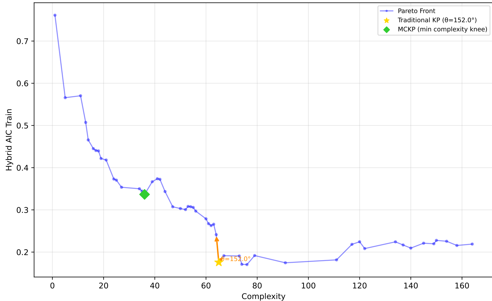
522_pm10 - Run 3 - SVP - Hybrid AIC Train \lambda_1=0.00, \lambda_2=0.10, \lambda_3=0.00 | Difficulty: 1.00 | Method: hmr
