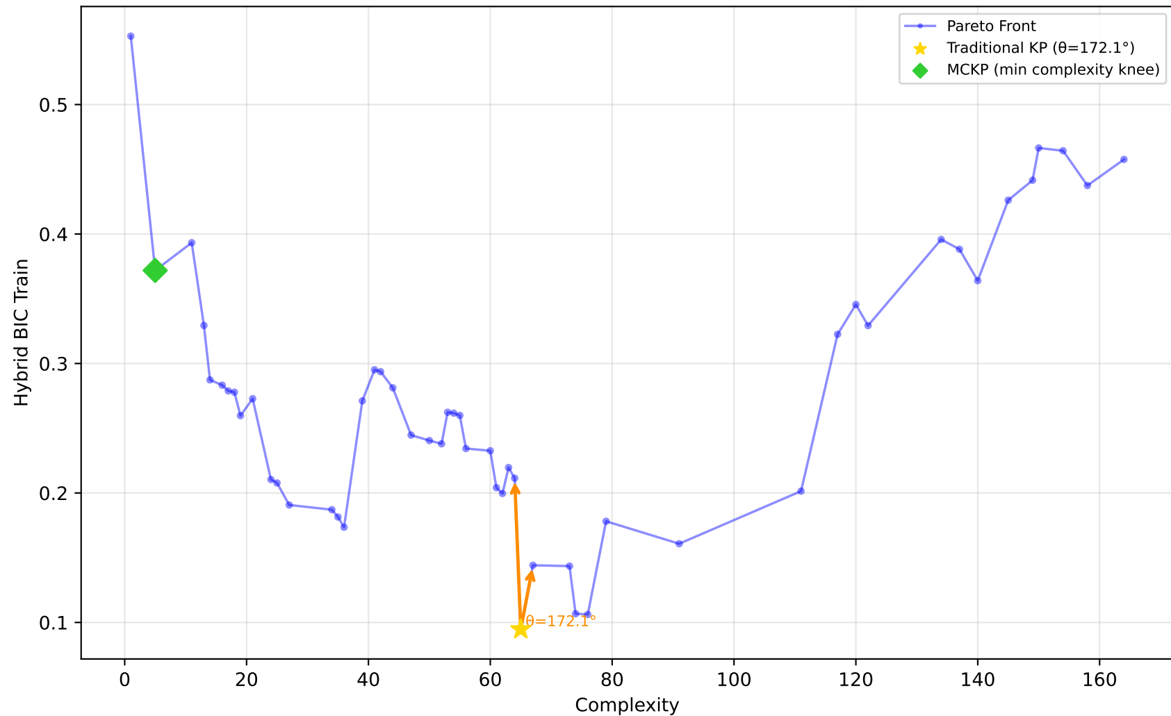
522_pm10 - Run 3 - SVP - Hybrid BIC Train \lambda_1=0.00, \lambda_2=0.10, \lambda_3=0.00 | Difficulty: 1.00 | Method: hmr
