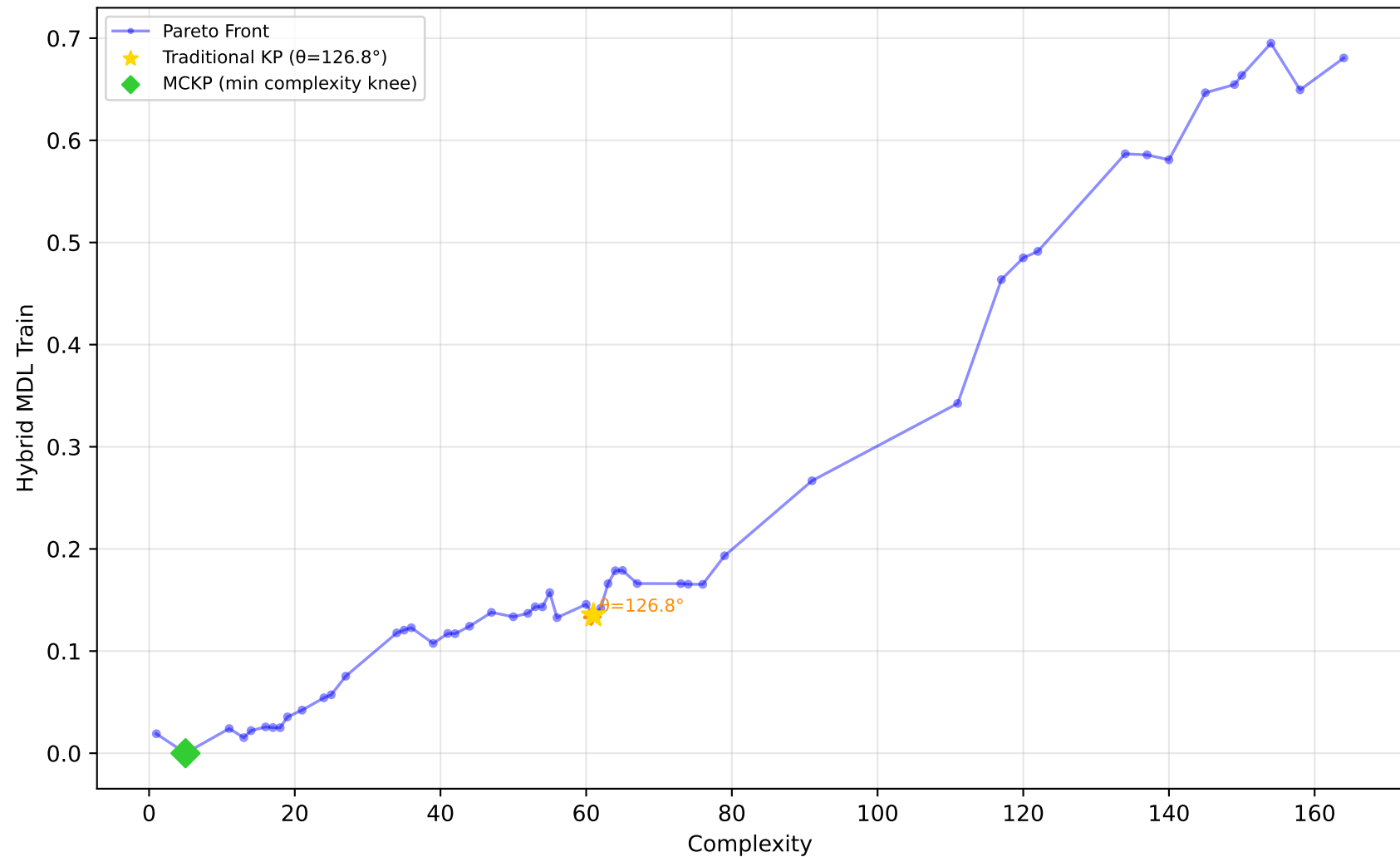
522_pm10 - Run 3 - SVP - Hybrid MDL Train \lambda_1=0.00, \lambda_2=0.10, \lambda_3=0.00 | Difficulty: 1.00 | Method: hmr
