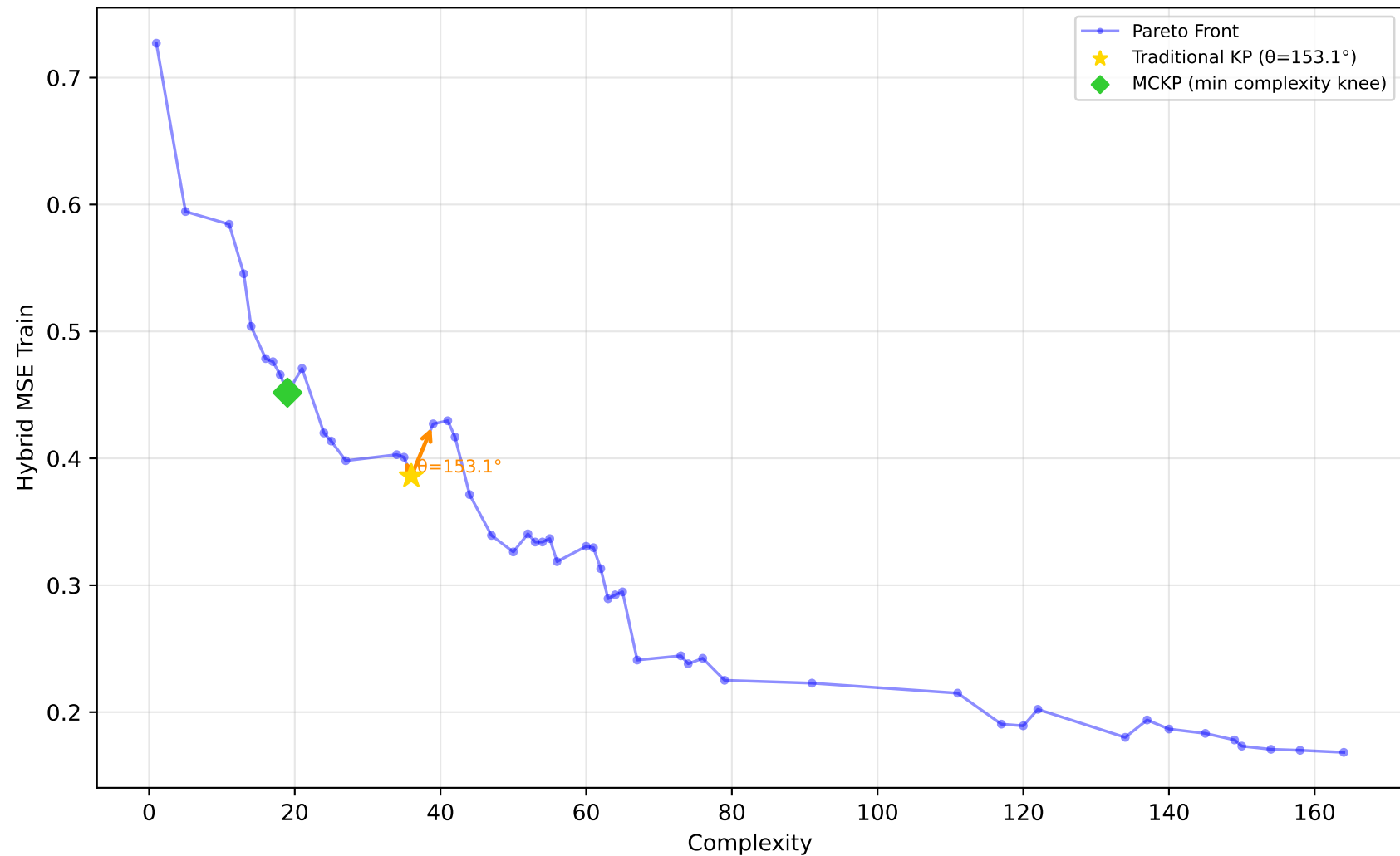
522_pm10 - Run 3 - SVP - Hybrid MSE Train \lambda_1=1.00, \lambda_2=0.00, \lambda_3=0.90 | Difficulty: 1.00 | Method: hmr
