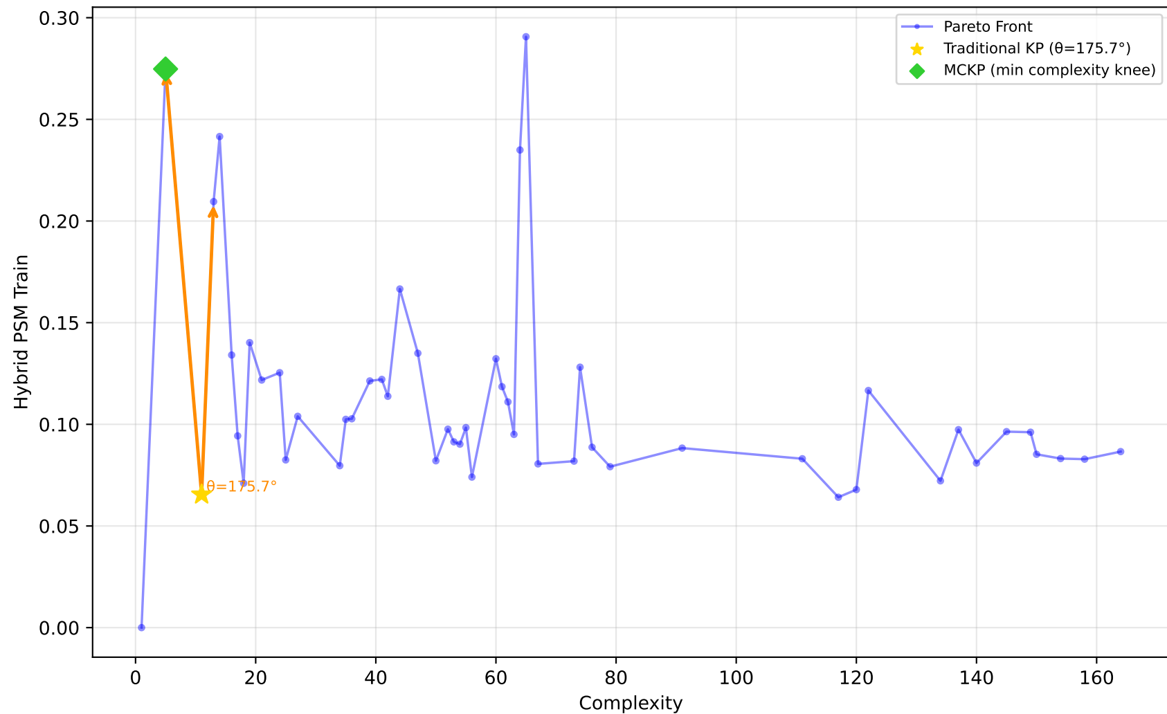
522_pm10 - Run 3 - SVP - Hybrid PSM Train \lambda_1=1.00, \lambda_2=0.00, \lambda_3=0.90 | Difficulty: 1.00 | Method: hmr
