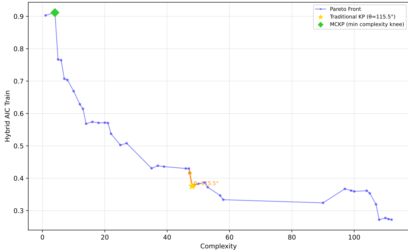
522_pm10 - Run 4 - MVP - Hybrid AIC Train \lambda_1=1.00, \lambda_2=0.00, \lambda_3=0.00 | Difficulty: 0.76 | Method: hmr
