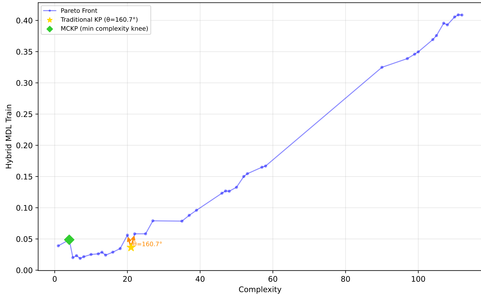
522_pm10 - Run 4 - MVP - Hybrid MDL Train \lambda_1=0.00, \lambda_2=0.90, \lambda_3=0.00 | Difficulty: 0.76 | Method: hmr
