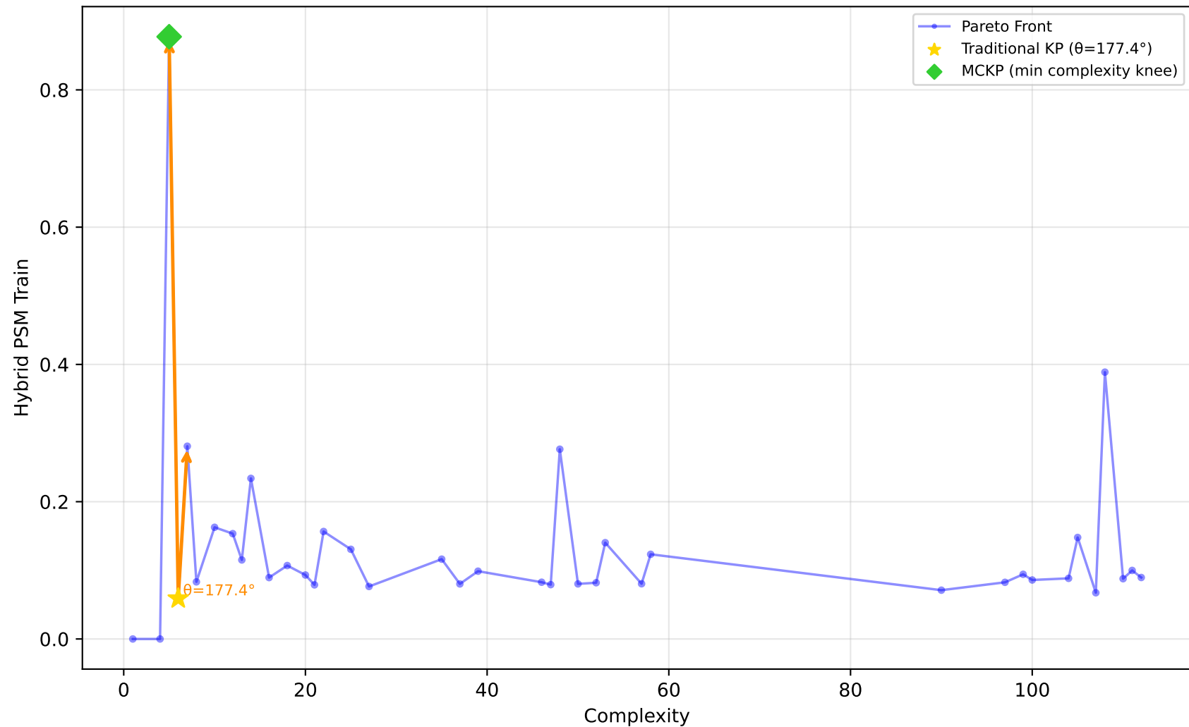
522_pm10 - Run 4 - MVP - Hybrid PSM Train \lambda_1=1.00, \lambda_2=0.00, \lambda_3=0.00 | Difficulty: 0.76 | Method: hmr
