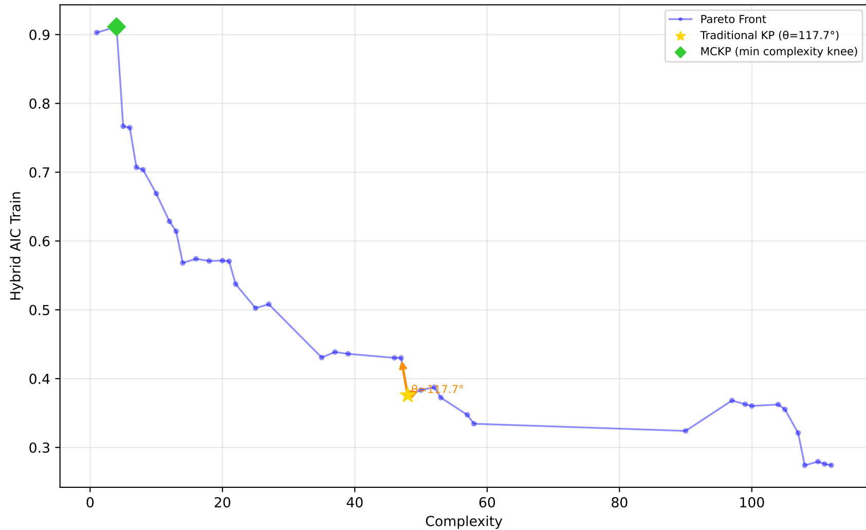
522_pm10 - Run 4 - SVP - Hybrid AIC Train \lambda_1=1.00, \lambda_2=0.00, \lambda_3=0.90 | Difficulty: 0.76 | Method: hmr
