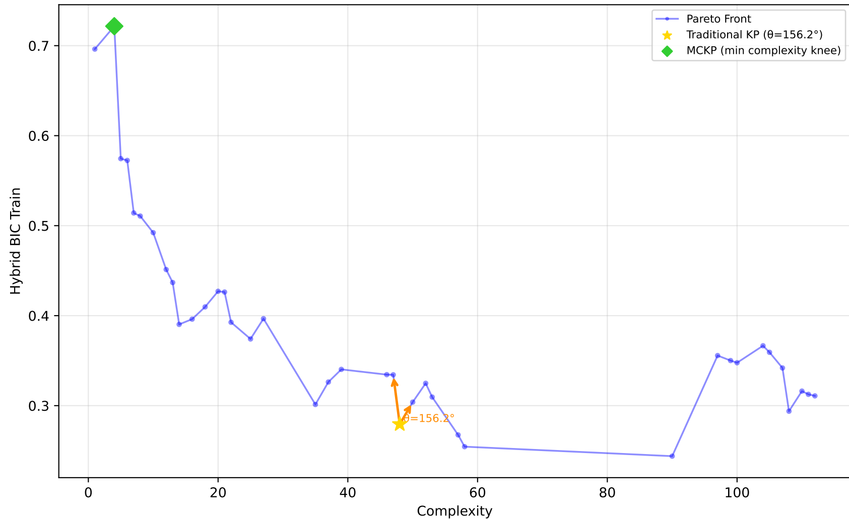
522_pm10 - Run 4 - SVP - Hybrid BIC Train \lambda_1=1.00, \lambda_2=0.00, \lambda_3=0.90 | Difficulty: 0.76 | Method: hmr
