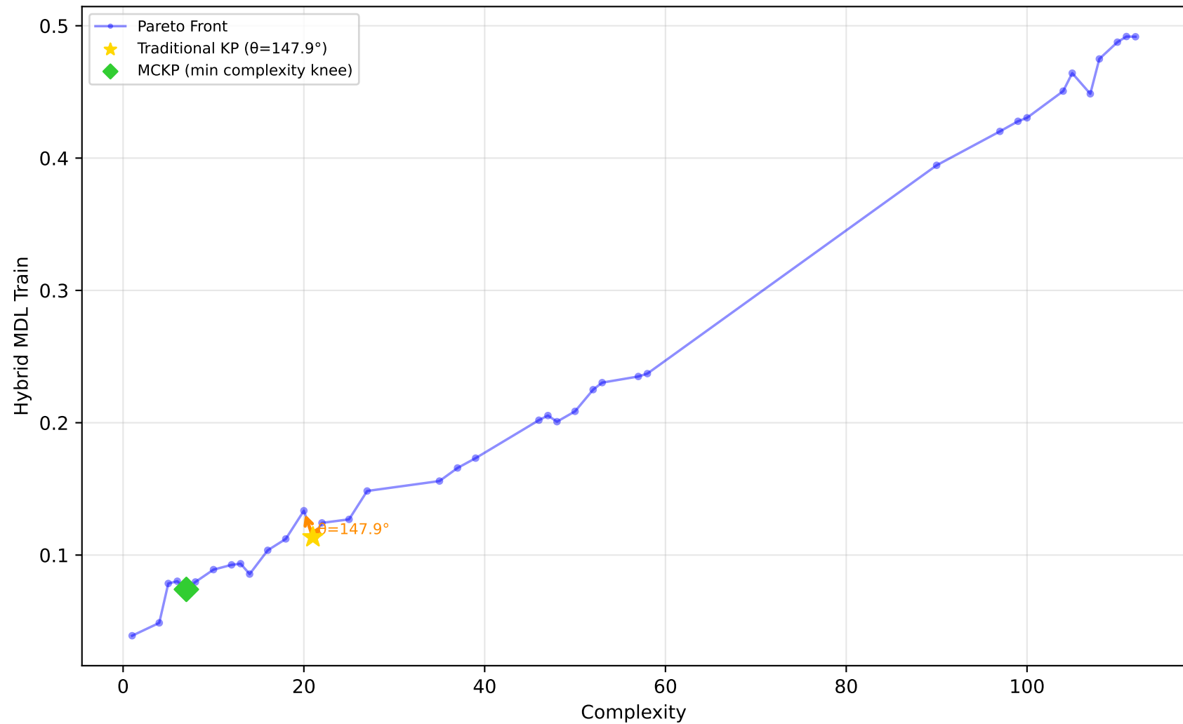
522_pm10 - Run 4 - SVP - Hybrid MDL Train \lambda_1=1.00, \lambda_2=0.00, \lambda_3=0.90 | Difficulty: 0.76 | Method: hmr
