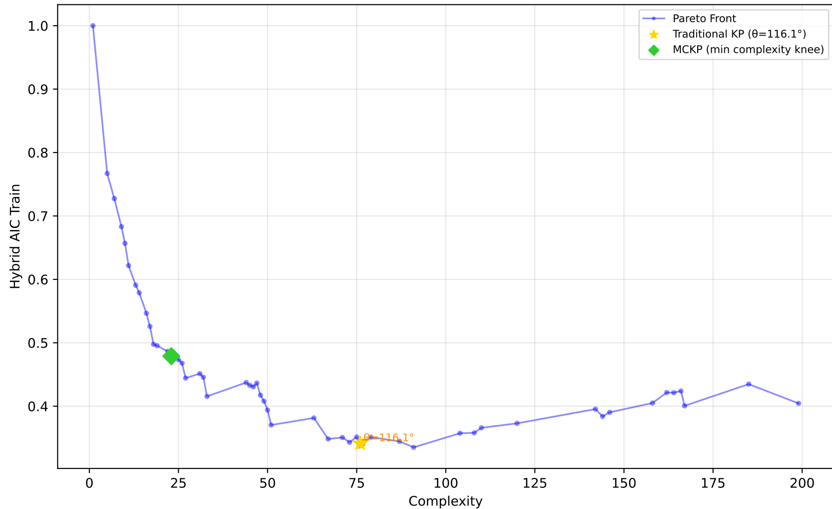
522_pm10 - Run 5 - MVP - Hybrid AIC Train \lambda_1=0.00, \lambda_2=0.90, \lambda_3=0.00 | Difficulty: 0.93 | Method: hmr
