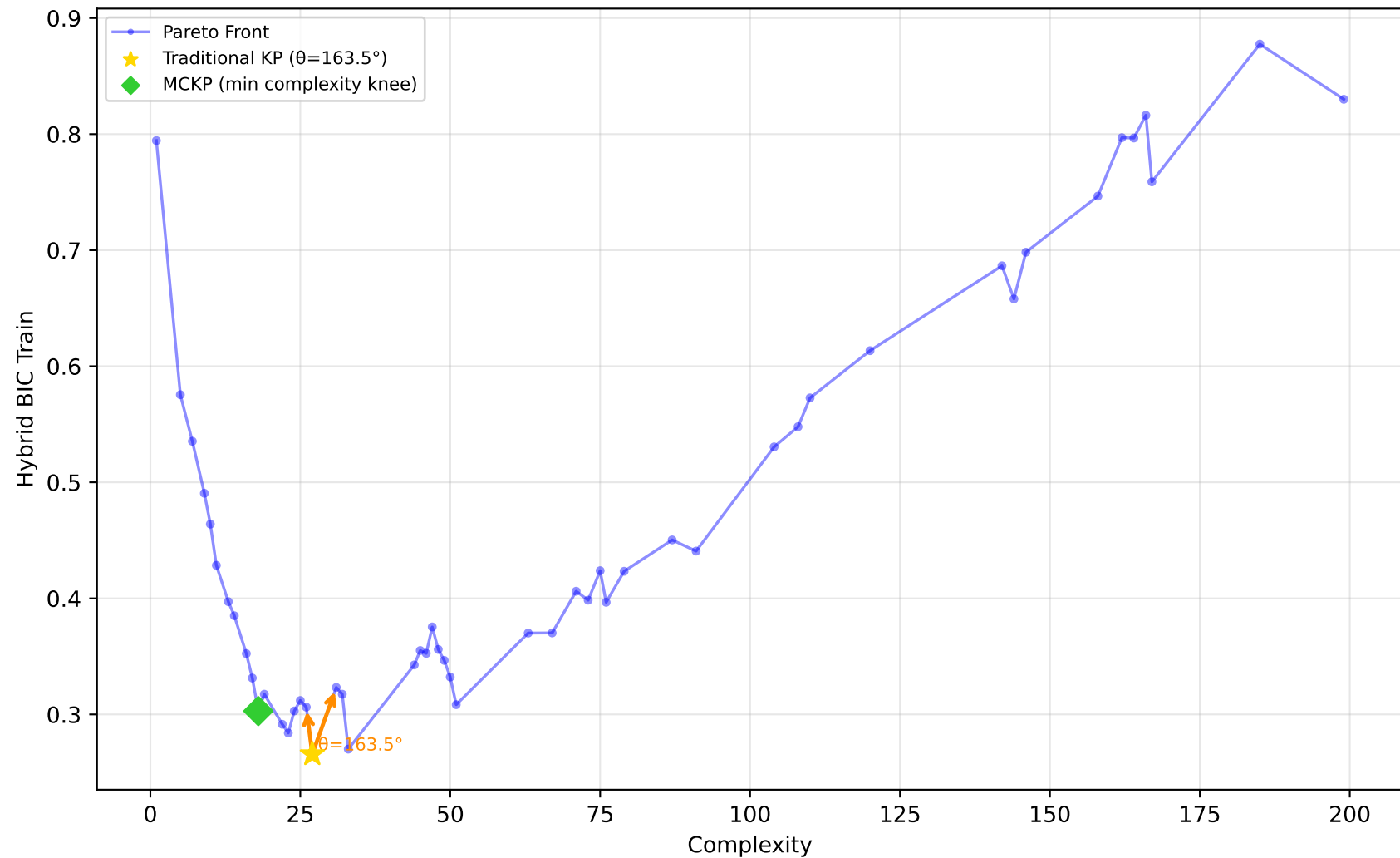
522_pm10 - Run 5 - MVP - Hybrid BIC Train \lambda_1=0.00, \lambda_2=0.90, \lambda_3=0.00 | Difficulty: 0.93 | Method: hmr
