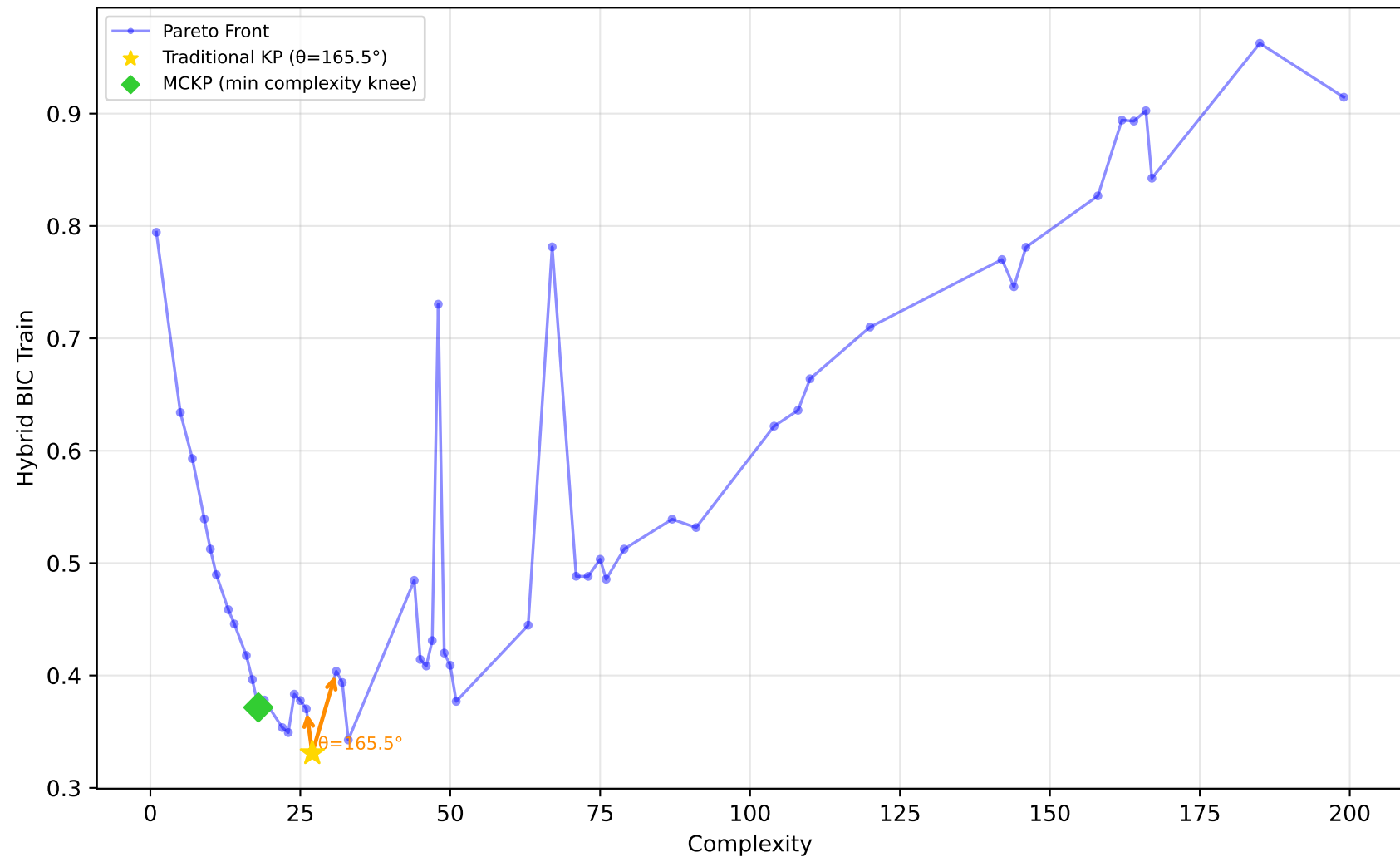
522_pm10 - Run 5 - MVP - Hybrid BIC Train \lambda_1=1.00, \lambda_2=0.00, \lambda_3=0.00 | Difficulty: 0.93 | Method: hmr
