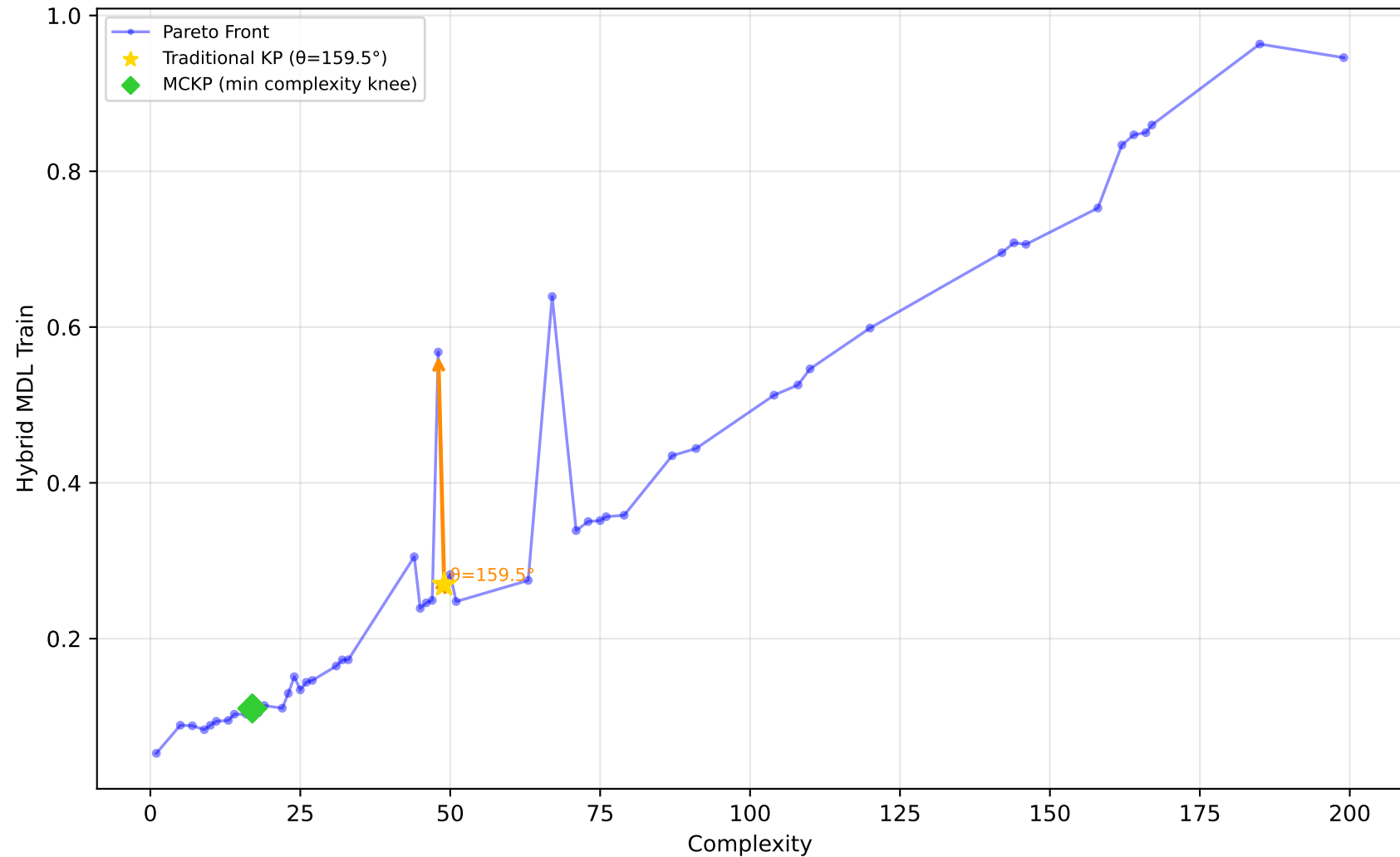
522_pm10 - Run 5 - MVP - Hybrid MDL Train \lambda_1=1.00, \lambda_2=0.00, \lambda_3=0.00 | Difficulty: 0.93 | Method: hmr
