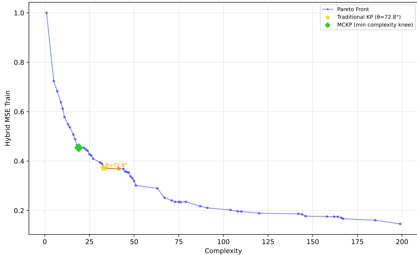
522_pm10 - Run 5 - MVP - Hybrid MSE Train \lambda_1=0.00, \lambda_2=0.90, \lambda_3=0.00 | Difficulty: 0.93 | Method: hmr
