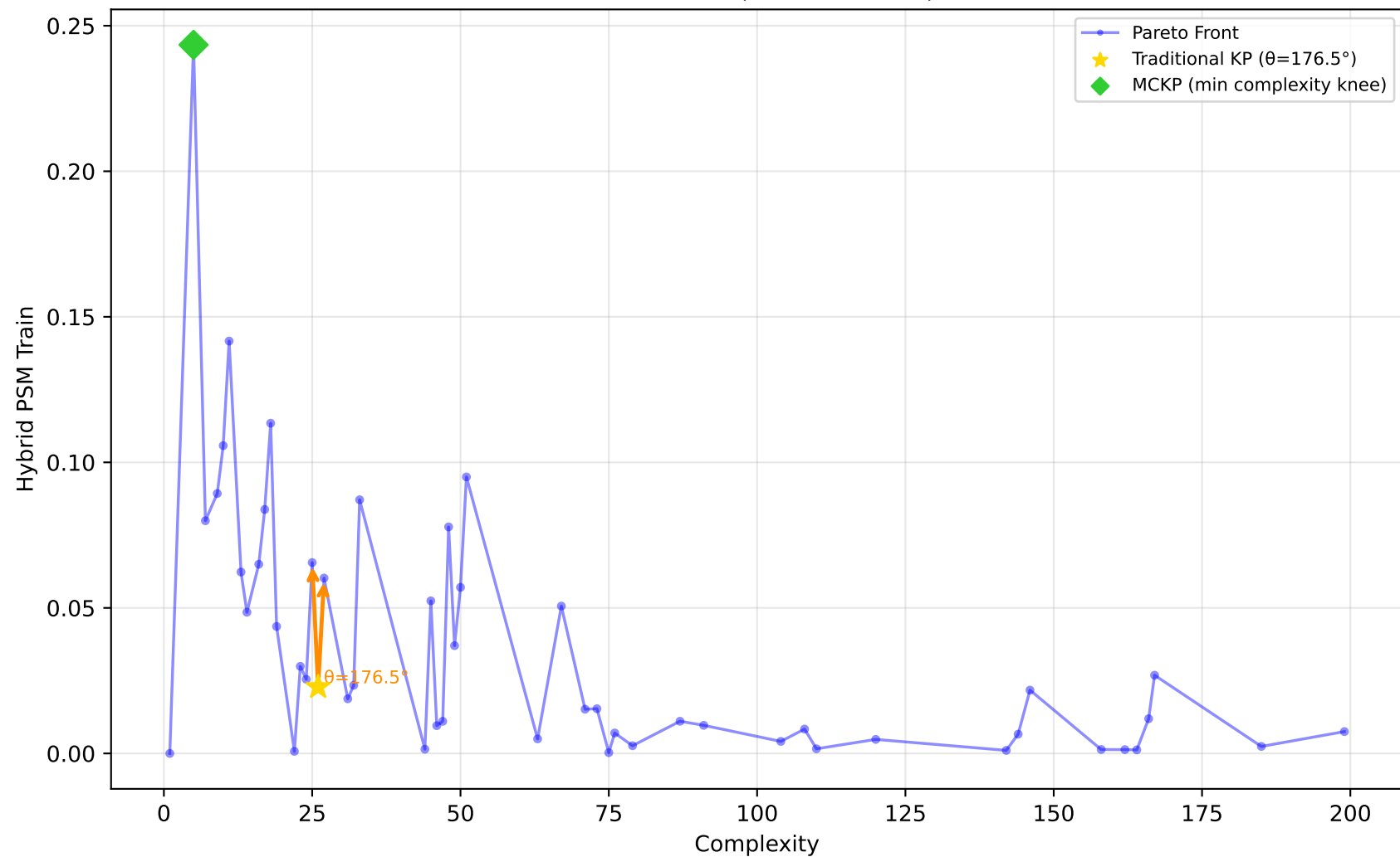
522_pm10 - Run 5 - MVP - Hybrid PSM Train \lambda_1=0.00, \lambda_2=0.90, \lambda_3=0.00 | Difficulty: 0.93 | Method: hmr
