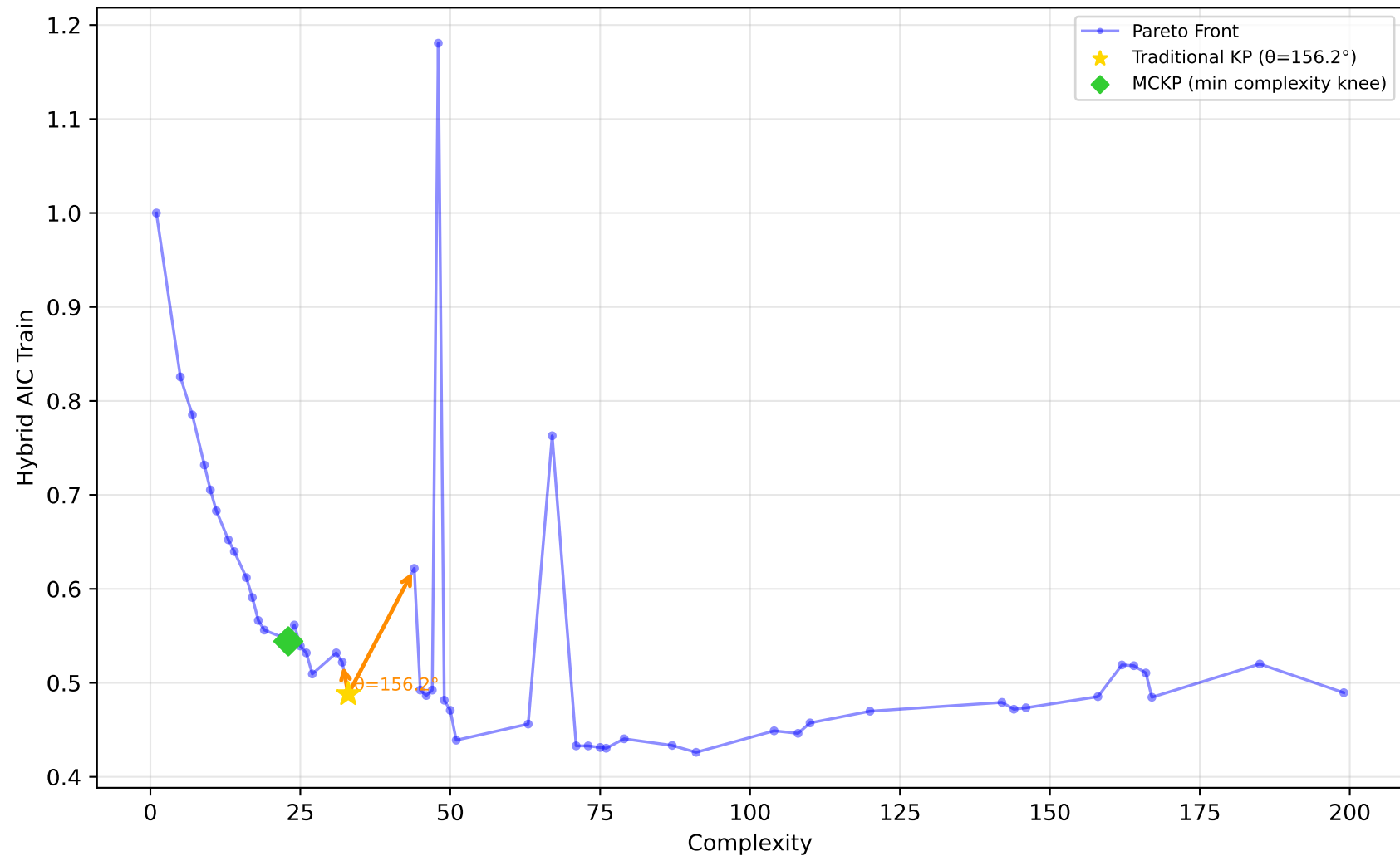
522_pm10 - Run 5 - SVP - Hybrid AIC Train \lambda_1=1.00, \lambda_2=0.00, \lambda_3=0.90 | Difficulty: 0.93 | Method: hmr
