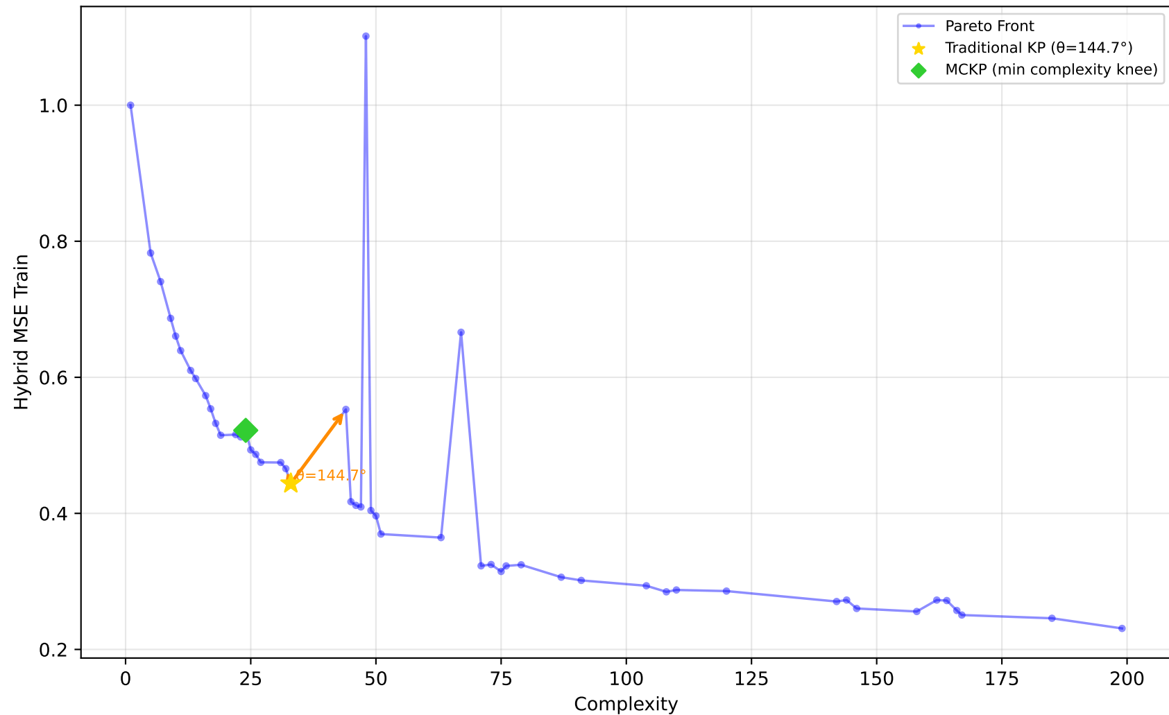
522_pm10 - Run 5 - SVP - Hybrid MSE Train \lambda_1=1.00, \lambda_2=0.00, \lambda_3=0.90 | Difficulty: 0.93 | Method: hmr
