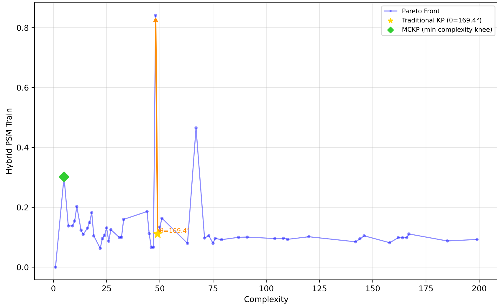
522_pm10 - Run 5 - SVP - Hybrid PSM Train \lambda_1=1.00, \lambda_2=0.00, \lambda_3=0.90 | Difficulty: 0.93 | Method: hmr
