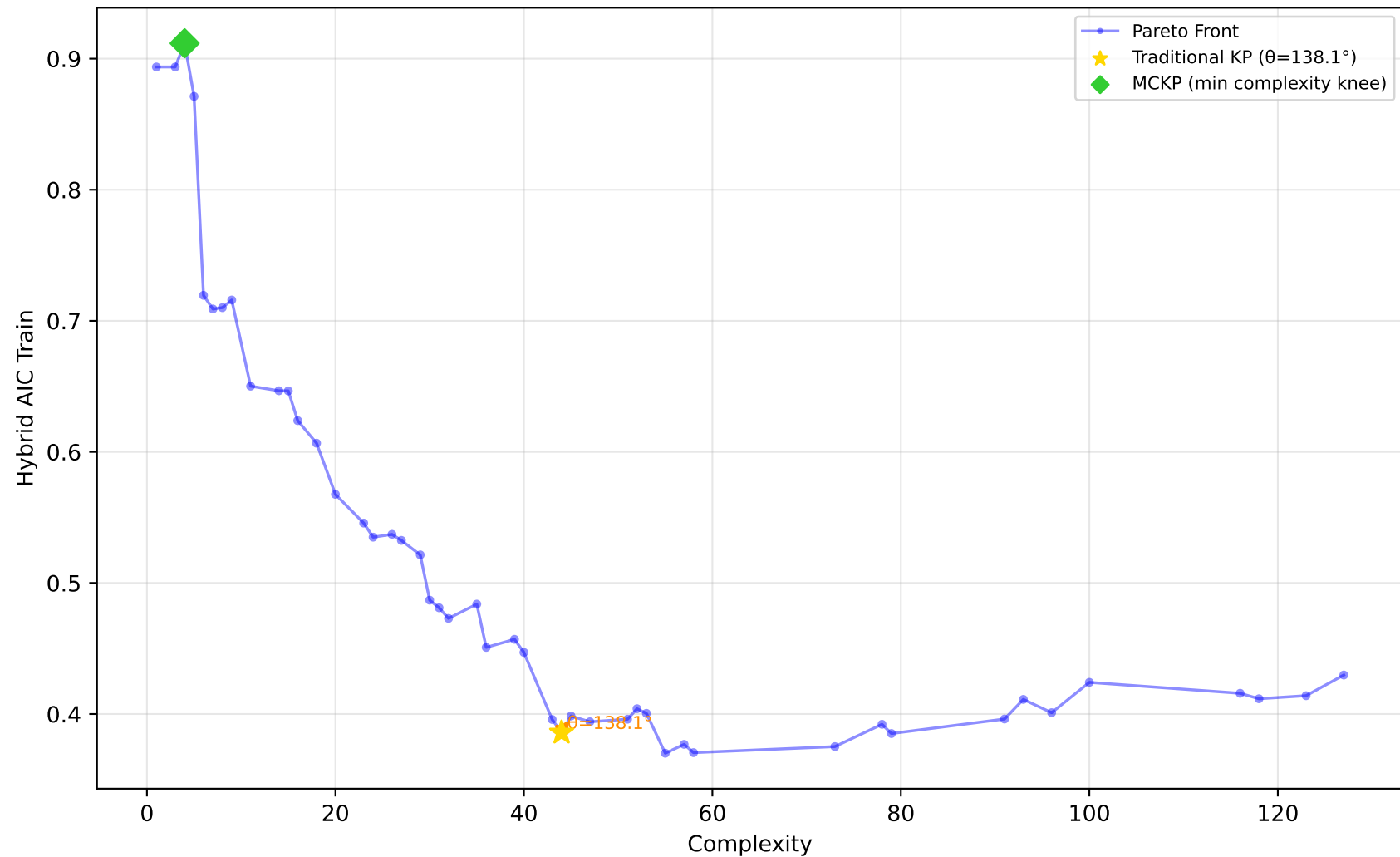
522_pm10 - Run 6 - MVP - Hybrid AIC Train \lambda_1=1.00, \lambda_2=0.00, \lambda_3=0.00 | Difficulty: 1.00 | Method: hmr
