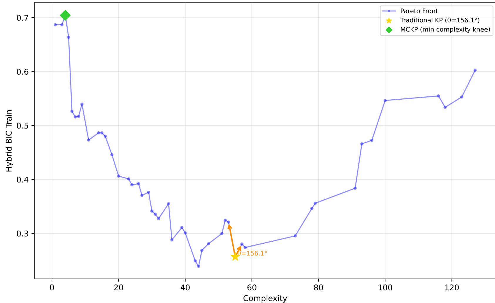
522_pm10 - Run 6 - MVP - Hybrid BIC Train \lambda_1=1.00, \lambda_2=0.00, \lambda_3=0.00 | Difficulty: 1.00 | Method: hmr
