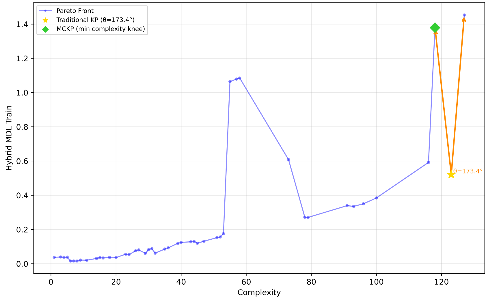
522_pm10 - Run 6 - MVP - Hybrid MDL Train \lambda_1=0.00, \lambda_2=0.90, \lambda_3=0.00 | Difficulty: 1.00 | Method: hmr
