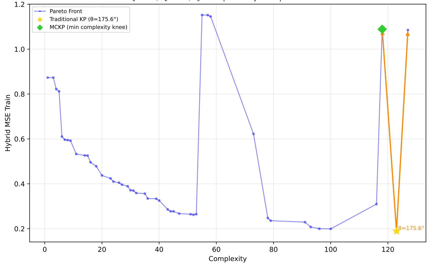
522_pm10 - Run 6 - MVP - Hybrid MSE Train \lambda_1=0.00, \lambda_2=0.90, \lambda_3=0.00 | Difficulty: 1.00 | Method: hmr
