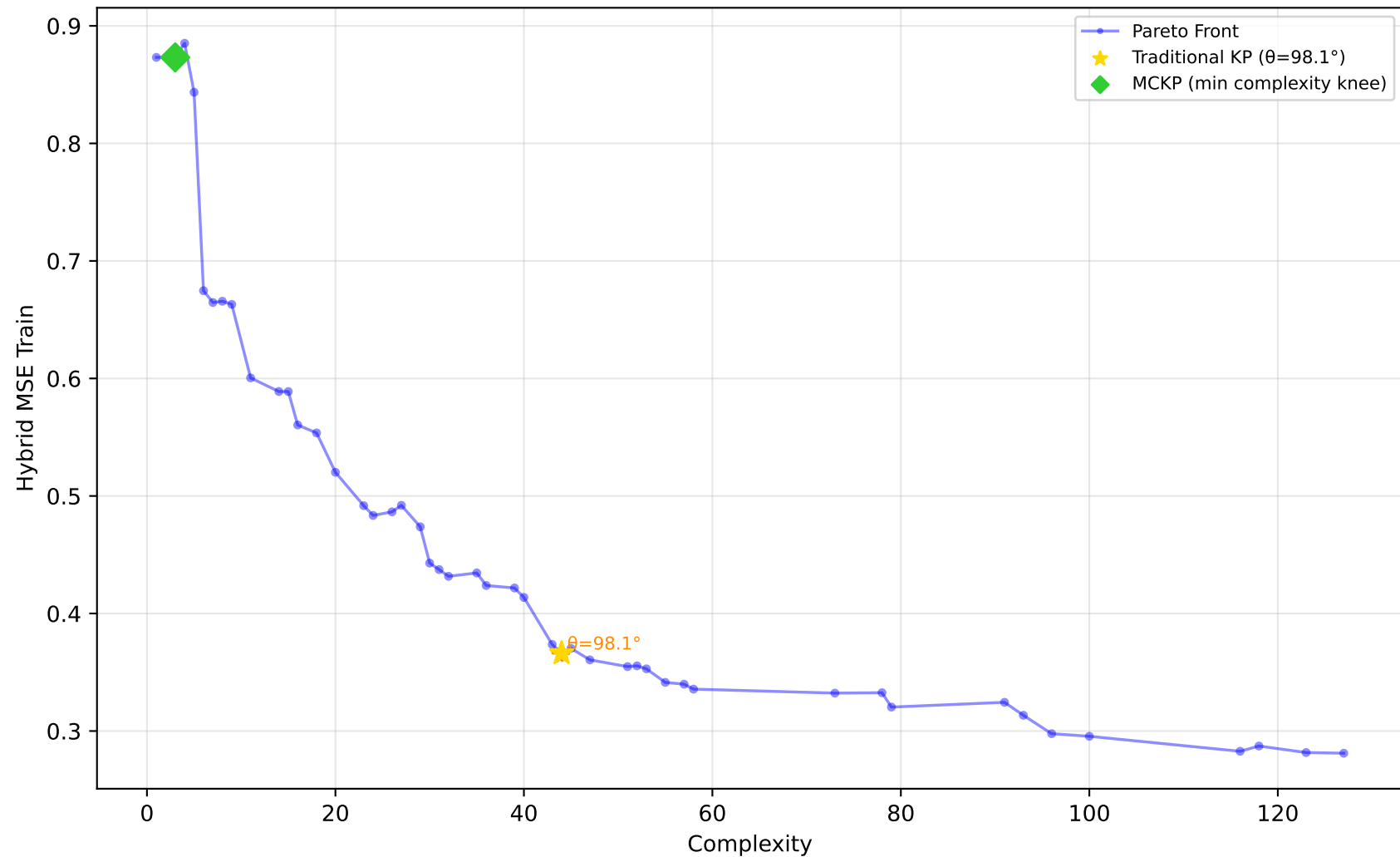
522_pm10 - Run 6 - MVP - Hybrid MSE Train \lambda_1=1.00, \lambda_2=0.00, \lambda_3=0.00 | Difficulty: 1.00 | Method: hmr
