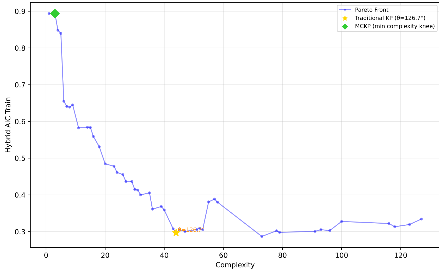
522_pm10 - Run 6 - SVP - Hybrid AIC Train \lambda_1=0.00, \lambda_2=0.10, \lambda_3=0.00 | Difficulty: 1.00 | Method: hmr
