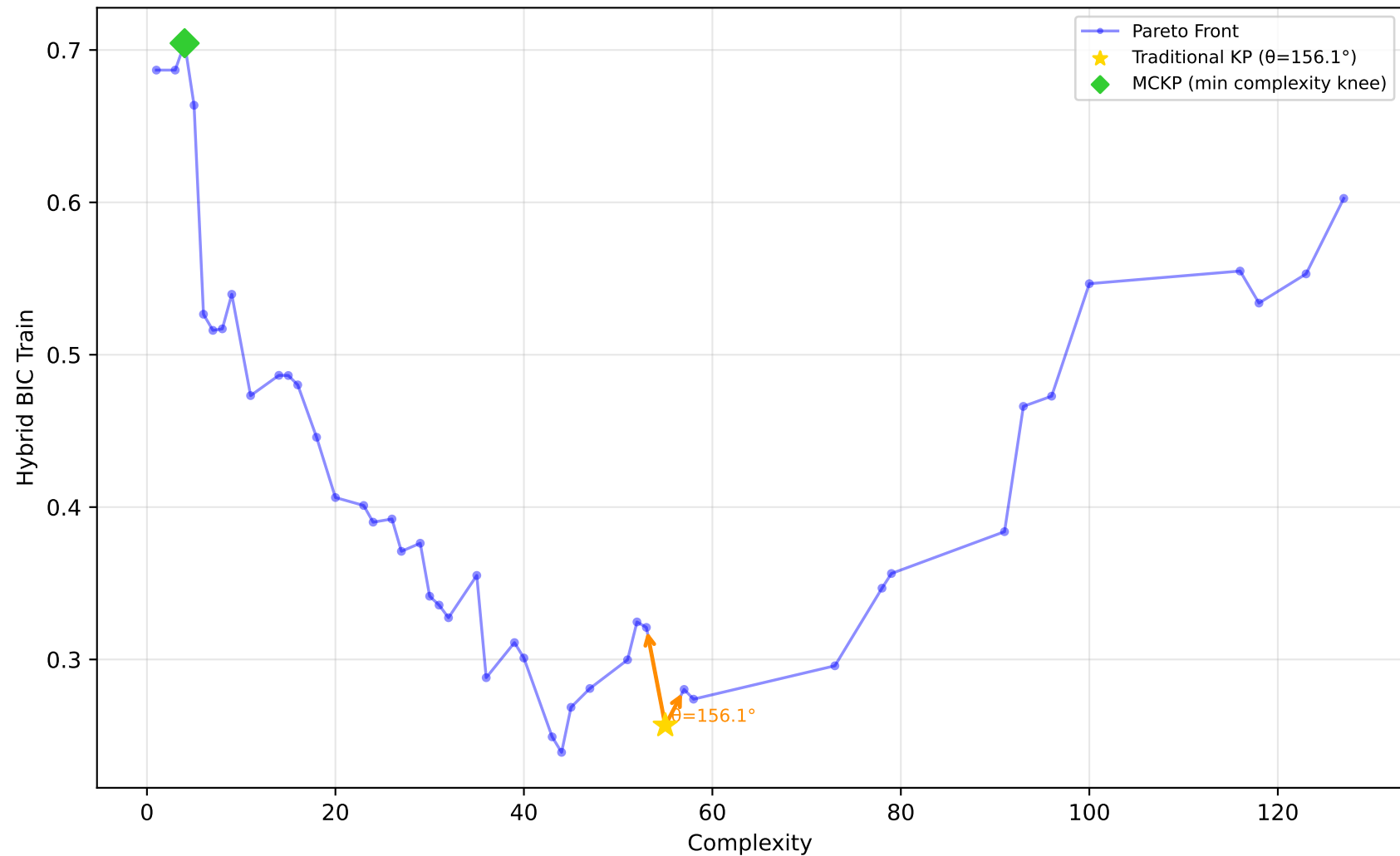
522_pm10 - Run 6 - SVP - Hybrid BIC Train \lambda_1=1.00, \lambda_2=0.00, \lambda_3=0.90 | Difficulty: 1.00 | Method: hmr
