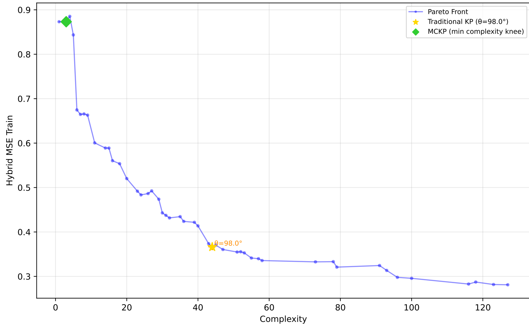
522_pm10 - Run 6 - SVP - Hybrid MSE Train \lambda_1=1.00, \lambda_2=0.00, \lambda_3=0.90 | Difficulty: 1.00 | Method: hmr
