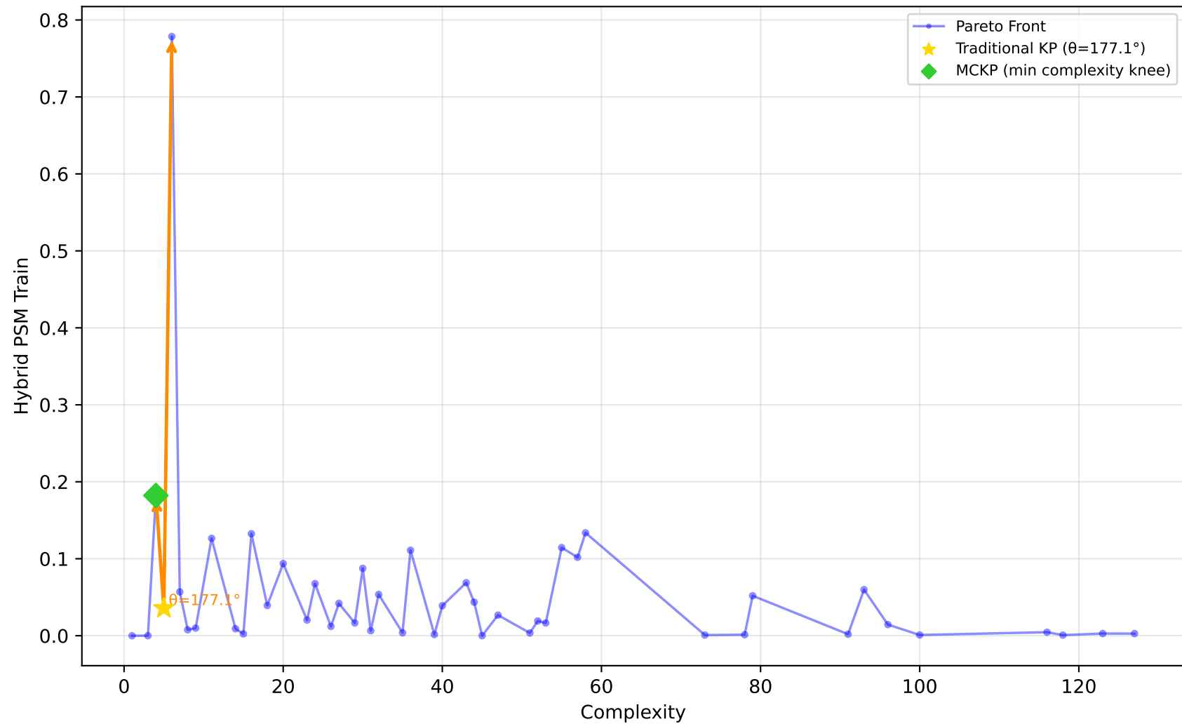
522_pm10 - Run 6 - SVP - Hybrid PSM Train \lambda_1=0.00, \lambda_2=0.10, \lambda_3=0.00 | Difficulty: 1.00 | Method: hmr
