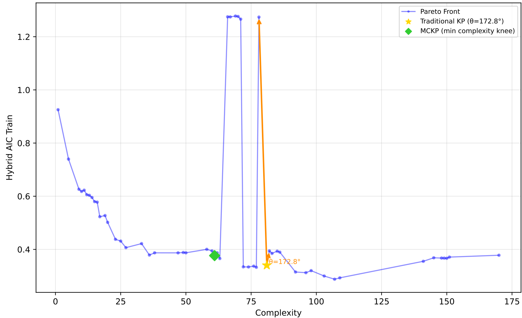
522_pm10 - Run 7 - MVP - Hybrid AIC Train \lambda_1=1.00, \lambda_2=0.00, \lambda_3=0.00 | Difficulty: 0.97 | Method: hmr
