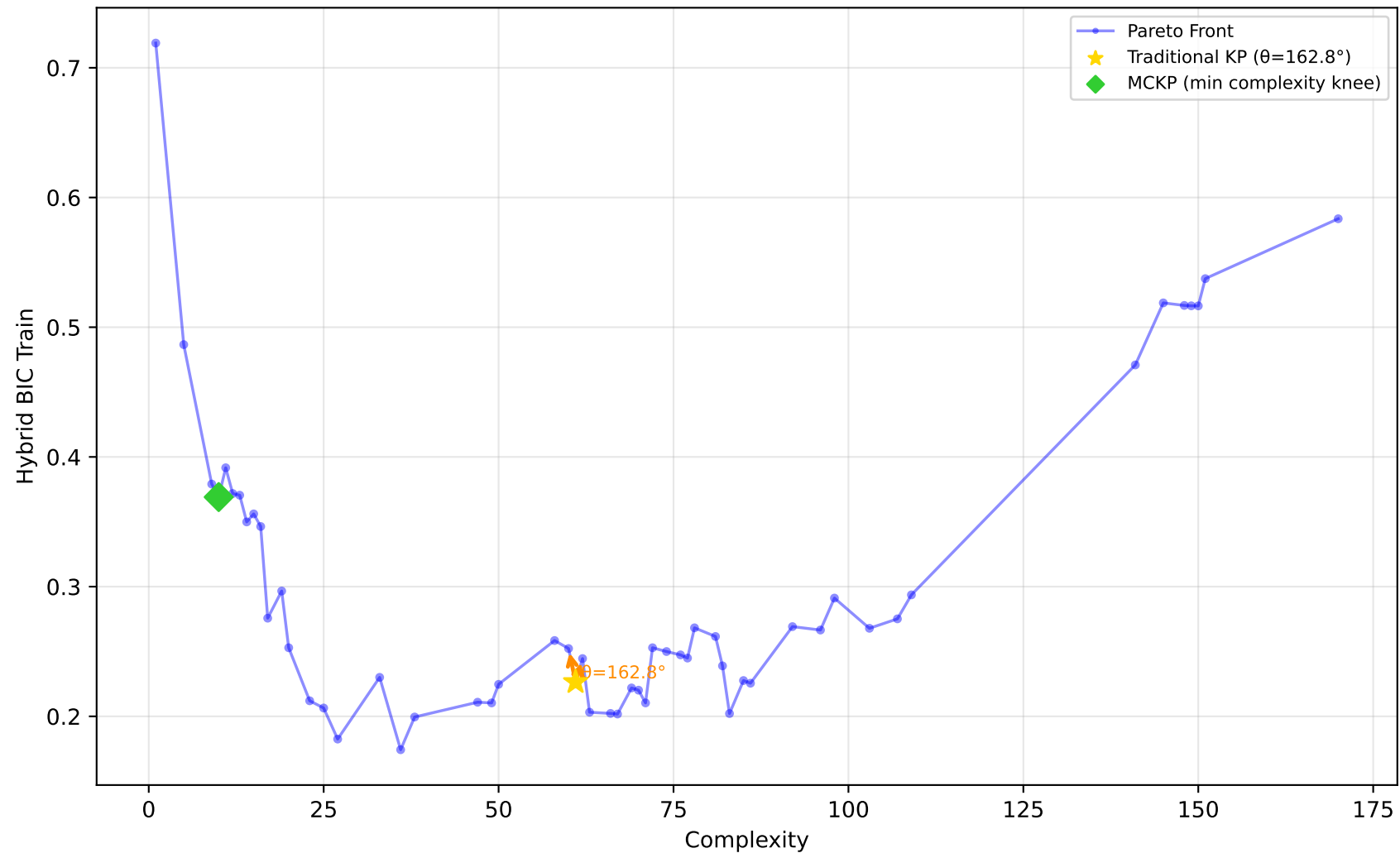
522_pm10 - Run 7 - MVP - Hybrid BIC Train \lambda_1=0.00, \lambda_2=0.90, \lambda_3=0.00 | Difficulty: 0.97 | Method: hmr
