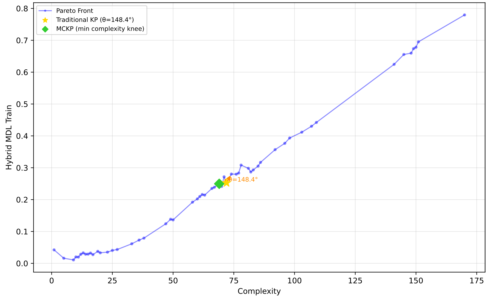
522_pm10 - Run 7 - MVP - Hybrid MDL Train \lambda_1=0.00, \lambda_2=0.90, \lambda_3=0.00 | Difficulty: 0.97 | Method: hmr
