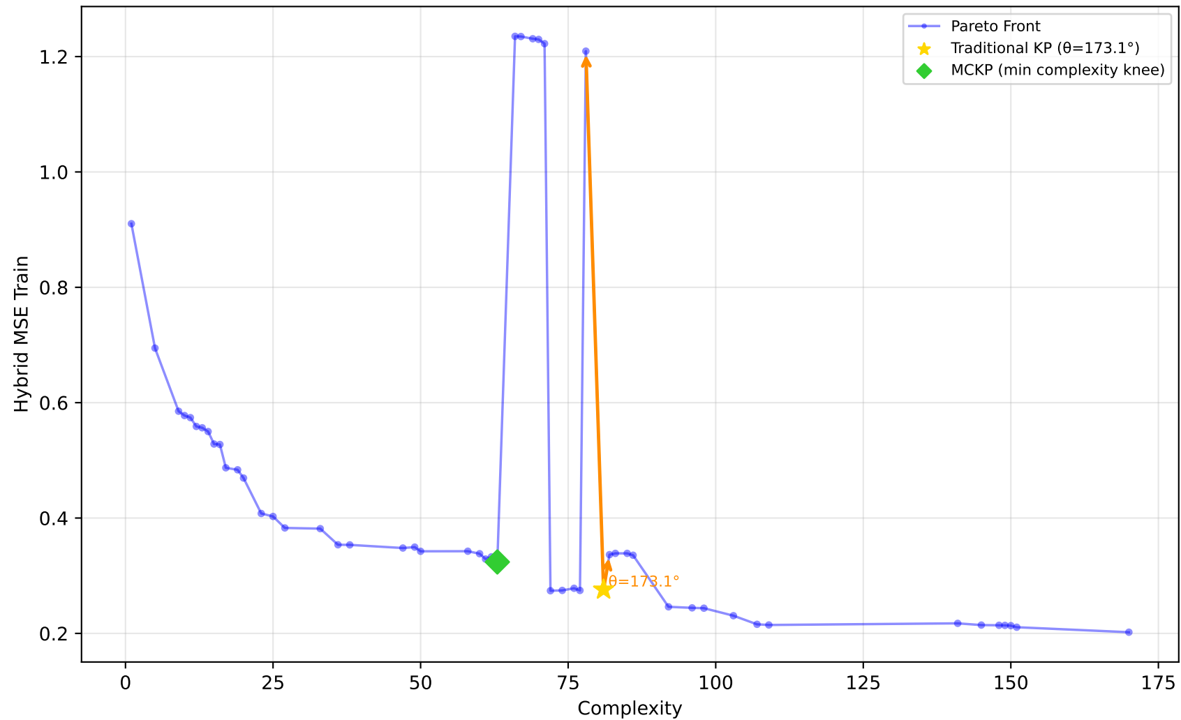
522_pm10 - Run 7 - MVP - Hybrid MSE Train \lambda_1=1.00, \lambda_2=0.00, \lambda_3=0.00 | Difficulty: 0.97 | Method: hmr
