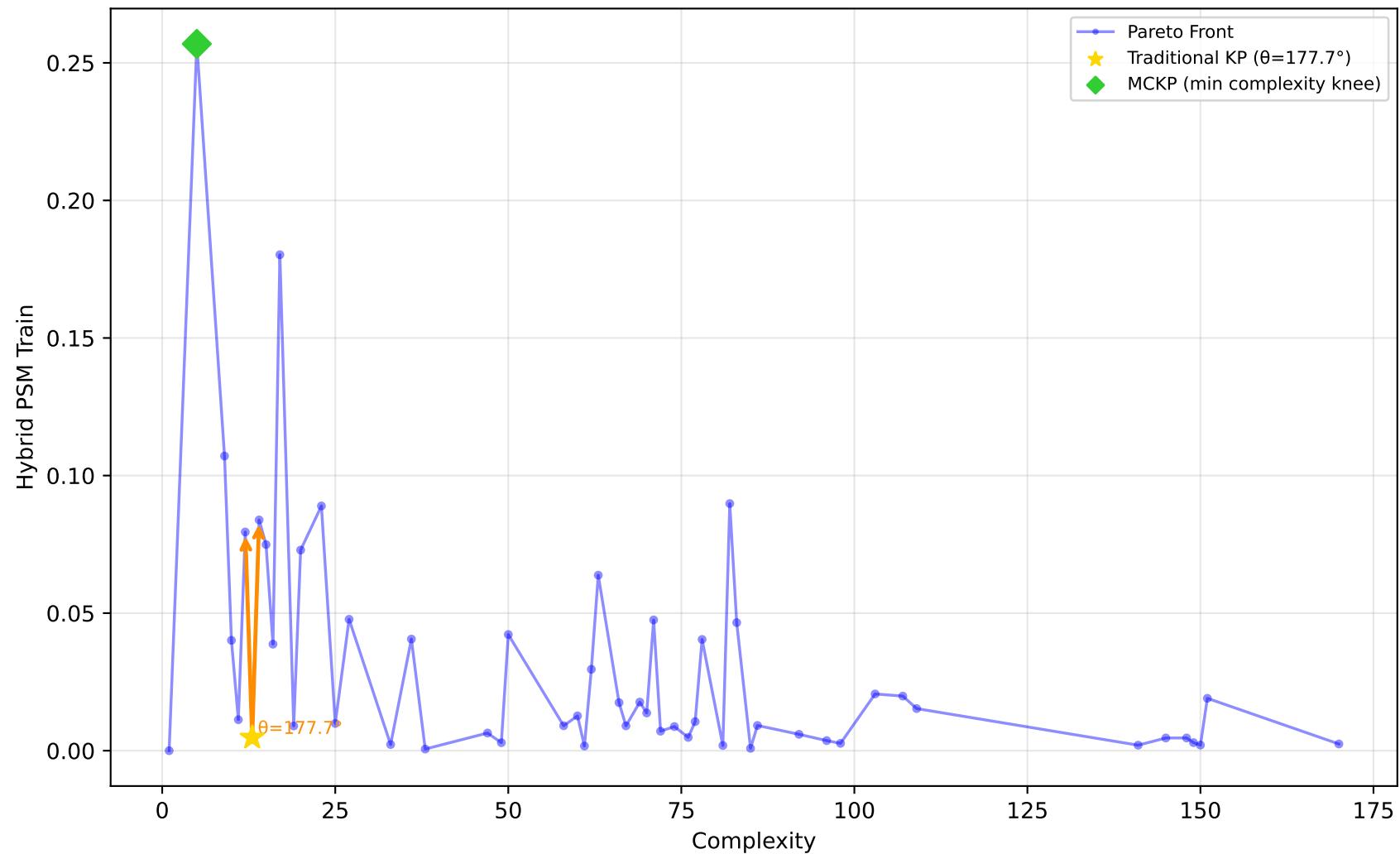
522_pm10 - Run 7 - MVP - Hybrid PSM Train \lambda_1=0.00, \lambda_2=0.90, \lambda_3=0.00 | Difficulty: 0.97 | Method: hmr
