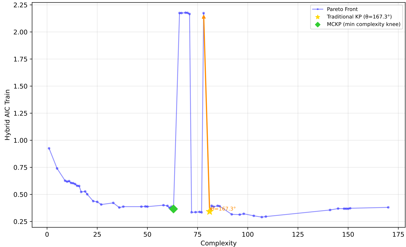
522_pm10 - Run 7 - SVP - Hybrid AIC Train \lambda_1=1.00, \lambda_2=0.00, \lambda_3=0.90 | Difficulty: 0.97 | Method: hmr
