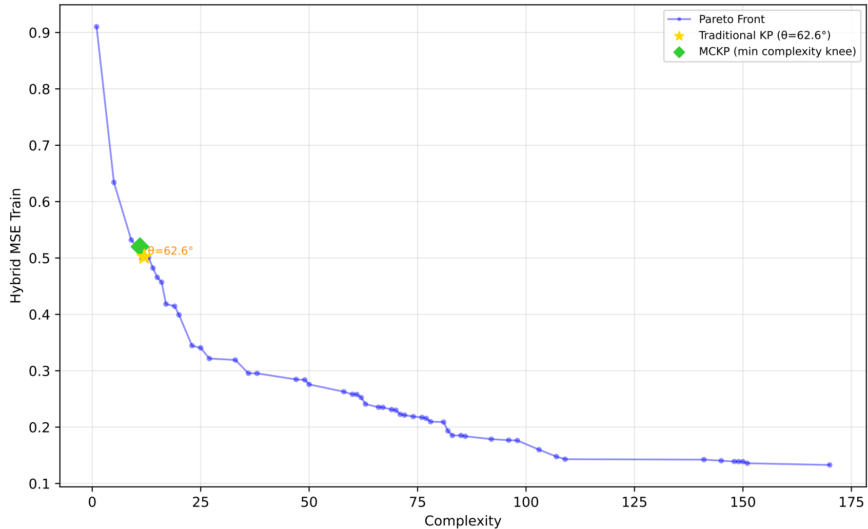
522_pm10 - Run 7 - SVP - Hybrid MSE Train \lambda_1=0.00, \lambda_2=0.10, \lambda_3=0.00 | Difficulty: 0.97 | Method: hmr
