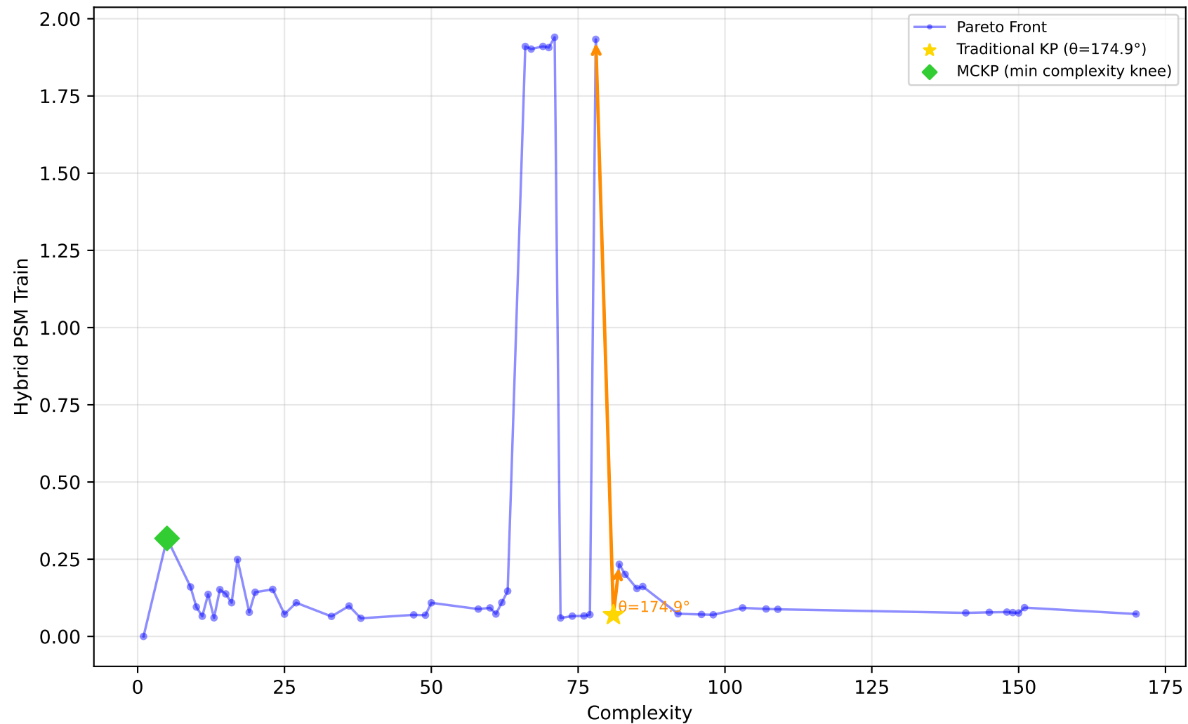
522_pm10 - Run 7 - SVP - Hybrid PSM Train \lambda_1=1.00, \lambda_2=0.00, \lambda_3=0.90 | Difficulty: 0.97 | Method: hmr
