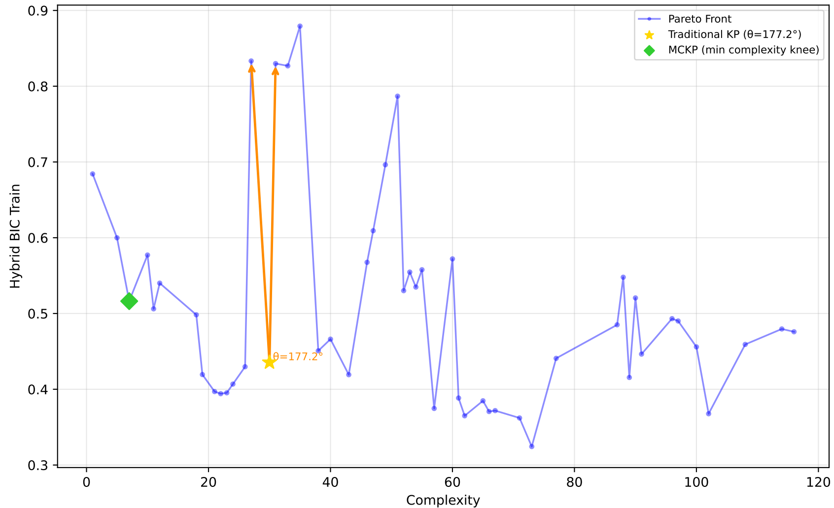
522_pm10 - Run 8 - MVP - Hybrid BIC Train \lambda_1=1.00, \lambda_2=0.00, \lambda_3=0.00 | Difficulty: 1.00 | Method: hmr
