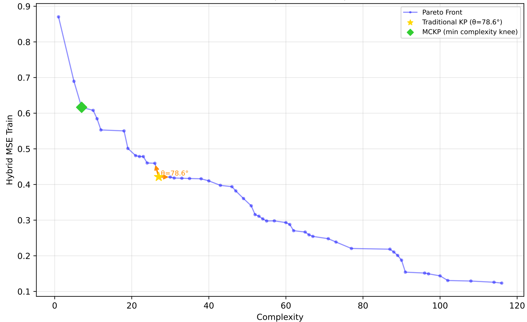
522_pm10 - Run 8 - MVP - Hybrid MSE Train \lambda_1=0.00, \lambda_2=0.90, \lambda_3=0.00 | Difficulty: 1.00 | Method: hmr
