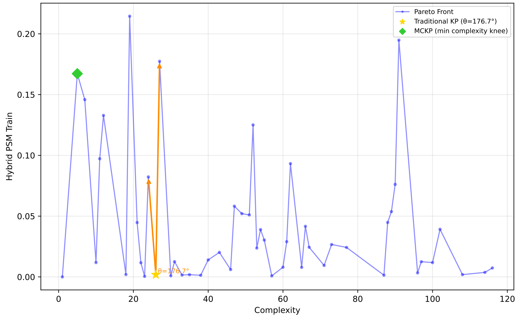
522_pm10 - Run 8 - MVP - Hybrid PSM Train \lambda_1=0.00, \lambda_2=0.90, \lambda_3=0.00 | Difficulty: 1.00 | Method: hmr
