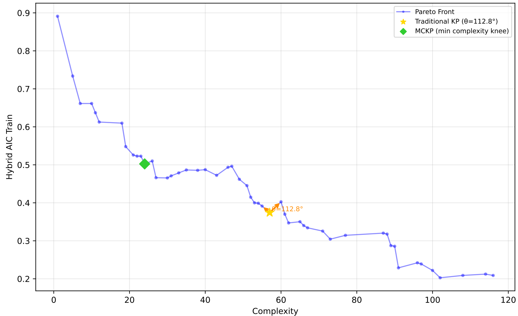
522_pm10 - Run 8 - SVP - Hybrid AIC Train \lambda_1=0.00, \lambda_2=0.10, \lambda_3=0.00 | Difficulty: 1.00 | Method: hmr
