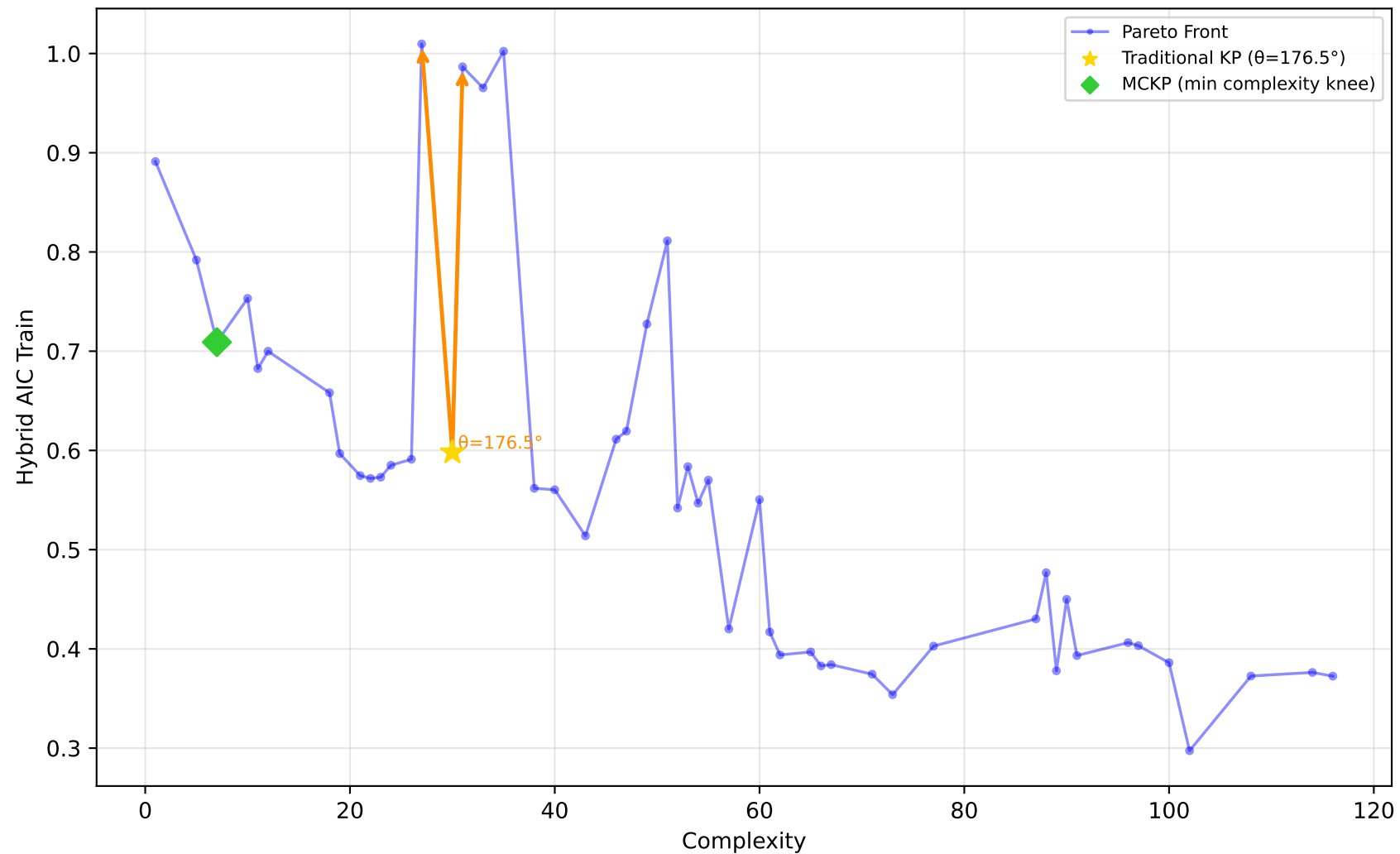
522_pm10 - Run 8 - SVP - Hybrid AIC Train \lambda_1=1.00, \lambda_2=0.00, \lambda_3=0.90 | Difficulty: 1.00 | Method: hmr
