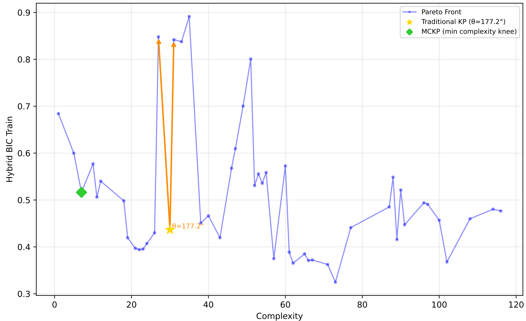
522_pm10 - Run 8 - SVP - Hybrid BIC Train \lambda_1=1.00, \lambda_2=0.00, \lambda_3=0.90 | Difficulty: 1.00 | Method: hmr
