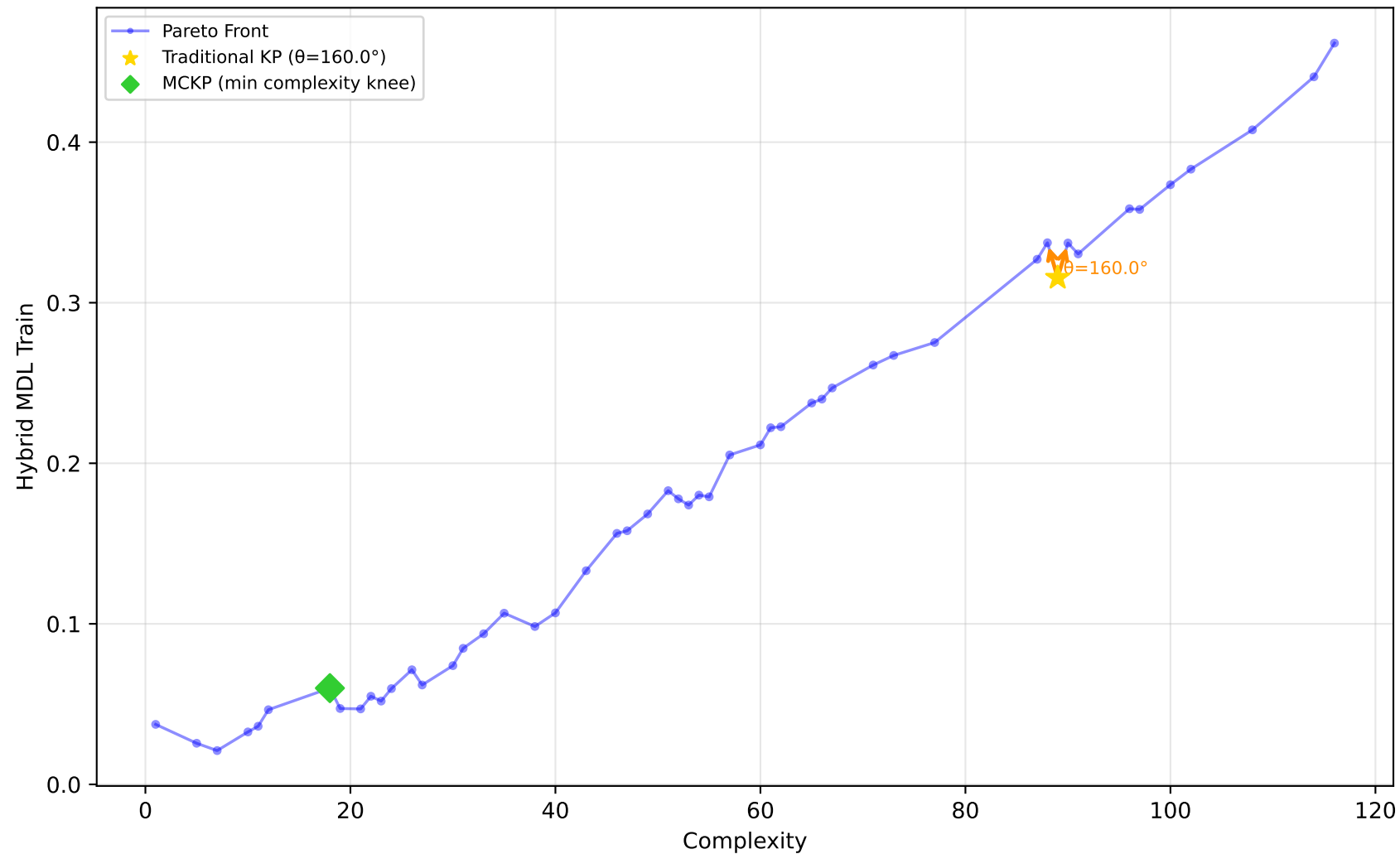
522_pm10 - Run 8 - SVP - Hybrid MDL Train \lambda_1=0.00, \lambda_2=0.10, \lambda_3=0.00 | Difficulty: 1.00 | Method: hmr
